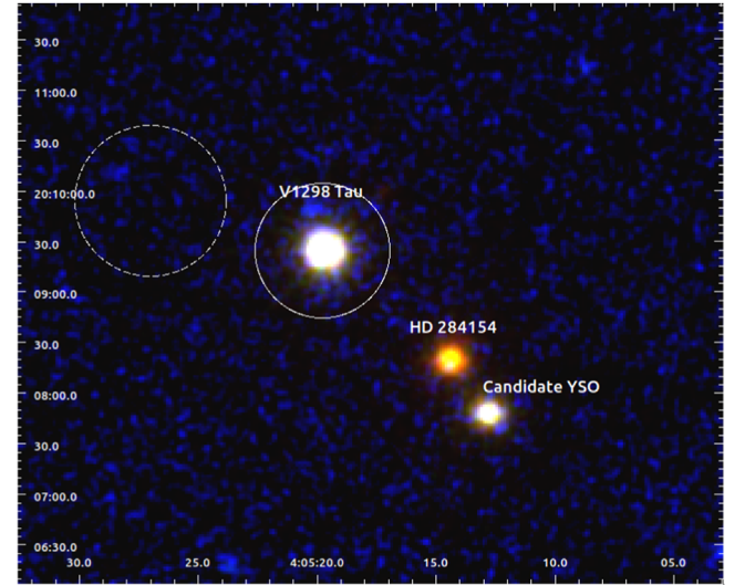
Figure 2. XMM-Newton EPIC red giant branch image of V1298 Tau. Red: 0.3–1.0 keV. Green: 1.0–3.0 keV. Blue: 3.0–8.0 keV. The target and the two bright nearby stars are labeled. The regions used for accumulating the spectra of V1298 Tau and the background are marked with white circles.
