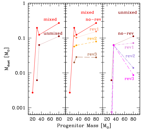
Figure 11. Left-hand panel: the mass of dust at the end of nucleation for mixed and unmixed ejecta for the four faint SN progenitors. Central panel: the mass of dust at the end of nucleation and after the passage of a reverse shock of increasing intensity for the four faint SN progenitors with mixed ejecta considered in this study. Right-hand panel: the same as in the central panel but for faint SN models with stratified ejecta. From top to bottom: no reverse shock models (no-rev), models with n_{ISM} = 0.06 (rev1), 0.6 (rev2) and 6 \text{ cm}^{-3} (rev3).
