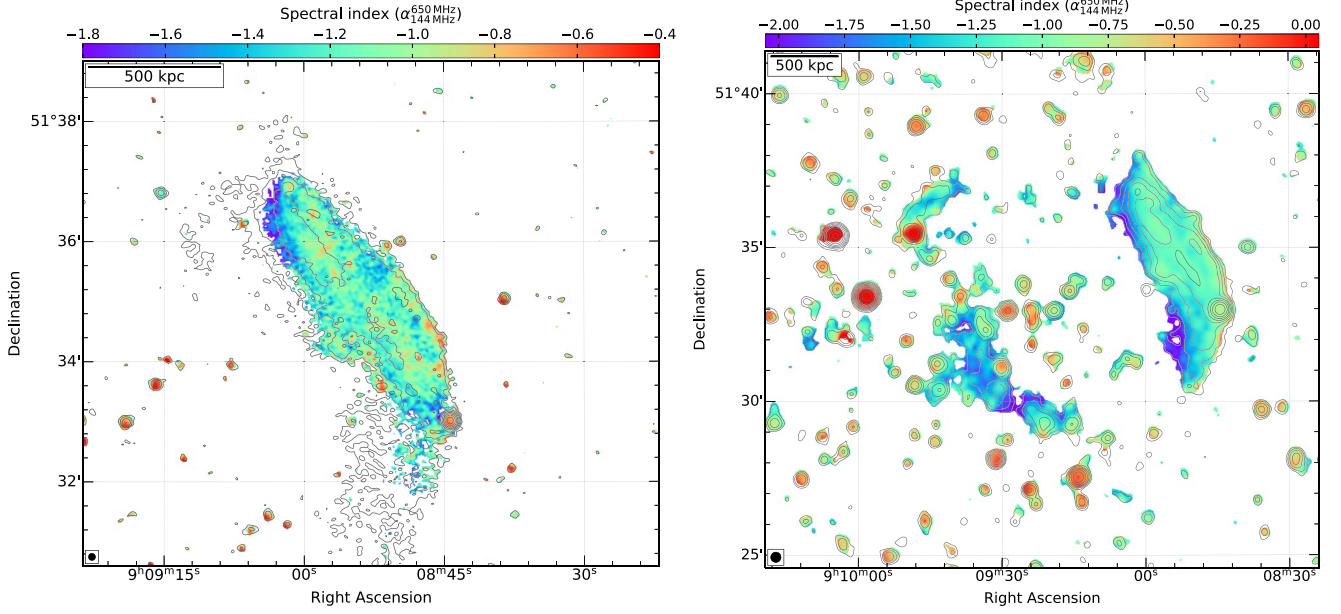
Figure 11. Left: spectral index map of the NW relic between 144 and 650 MHz at 7'' resolution. Right: spectral index map of A746 at 20'' resolution. Black contours are drawn at levels of [1, 2, 4, 8, \dots] \times 4.0\sigma_{\text{rms}} and are from the LOFAR 144 MHz image. Pixels with values below 3.0\sigma_{\text{rms}} maps were blanked. The image properties are given in Table 2, for IM2, IM5, IM4, and IM8.
