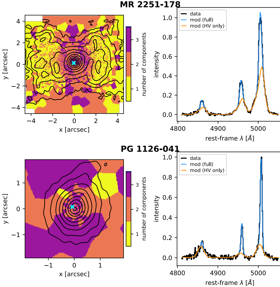
Fig. 3. Multi-component fit for diffuse gas emission lines of MR 2251–178 (top panels) and PG 1126–041 (bottom panels). Left-hand panels: iso-intensity contours for the integrated [O III] line (black lines); the background colours show the number of components used in each Voronoi bin. The [O III] maps are derived by integrating the (unbinned) BLR-subtracted cubes in the \lambda\lambda 4930 – 5030 Å rest-frame range and are spatially smoothed to a FWHM resolution of 0.25'' . Contours are spaced by a factor of 2, the outermost being at 3\times the rms noise. The crosses in cyan mark the bins at which the spectra shown in the right panels are extracted. Right-hand panels: representative spectra in a range encompassing the H \beta and [O III] lines for the BLR-subtracted cubes (black lines), our best-fit models (blue lines), and their HV sub-components alone (orange lines).
