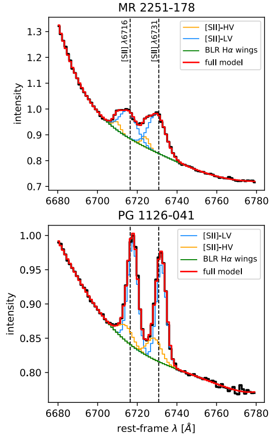
Fig. 5. [S II] emission lines and related models for MR 2251–178 (top panel) and PG 1126–041 (bottom panel). The black lines show the spectrum extracted within an aperture of 0.05'' (for MR 2251–178) and 0.5'' (for PG 1126–041) from the systems’ nuclei. The red lines show our best-fit models, with separate contributions from the wings of the BLR H \alpha (green lines), and the HV- and LV-components of the [S II] doublets (orange and blue lines, respectively).
