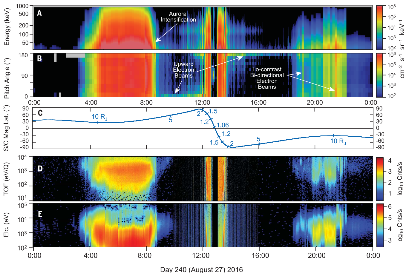
Fig. 3. Electron and ion observations obtained during Juno's
