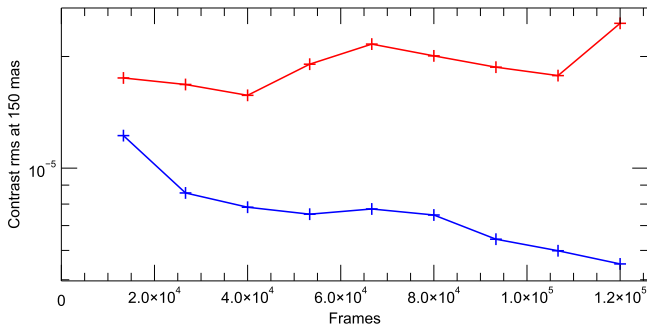
Figure 8. ADI (red) and SFADI (blue) contrast rms of background residuals photometry as a function of the number of frames of the acquisition sequence. Note that a subset of 1 frame every 10 has been used here to speed up the computation time.
