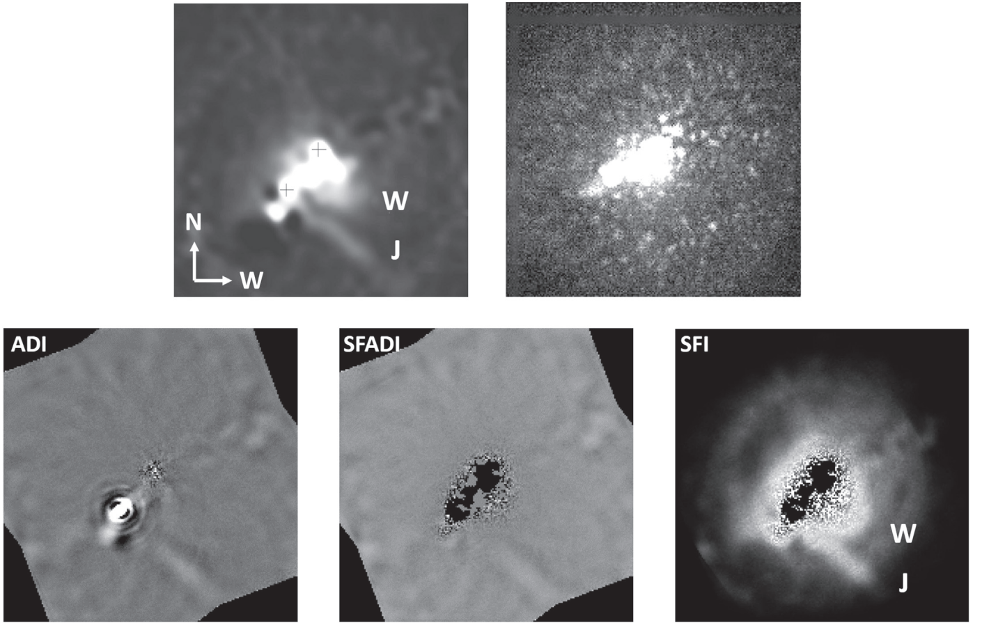
Figure 9. Extended circumstellar structure ( 10^{-4} contrast) around the ZCMa binary (whose flux-scaled model, based on Antonucci et al. 2016, is shown in the top-left panel) as viewed after convolution with the PSF of a single frame of the SHARK-VIS Forerunner sequence (top-right). In the bottom panels, the results of the application of ADI, SFADI, and SFI methods are shown (from left to right, respectively). The W and J labels indicate the wide wind from the primary NW component, and the collimated jet from the secondary star, respectively.
