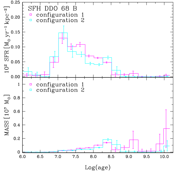
Figure 16. SFHs for stars in magenta and cyan in Figure 15. Notice that in this case the SFRs are multiplied by 100.
