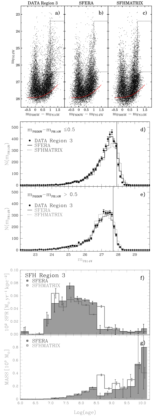
Figure 13. Same as Figures 11 and 12 but for Region 3. Notice that in this case the SFRs of panel (f) are multiplied by 100.
