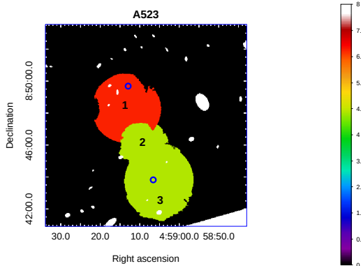
Figure 14. Temperature map (keV) showing that the northern cluster region is characterized by a higher temperature than the central and southern regions. The central 1.5' radius region, indicated by the label “2”, is centred close to the X-ray peak, precisely at R.A.=04 h 59 m 09 s .0, Dec.=+08°45'55" (J2000.0). The FOW of the image is \sim 1.5 \times 1.5 h_{70}^{-1} Mpc. The two small blue circles indicate BCG1 and BCG2 in the northern and southern regions (regions 1 and 3, respectively).
