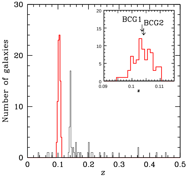
Figure 4. Redshift galaxy distribution. Thick red line histogram refers to the 80 galaxies assigned to A523 according to the 1D-DEDICA reconstruction method. An important background structure at z \sim 0.14 (BACKstruct) is also evident in the figure. The inset figure shows the member-galaxy distribution with the indication of the BCG1 and BCG2 velocities.
