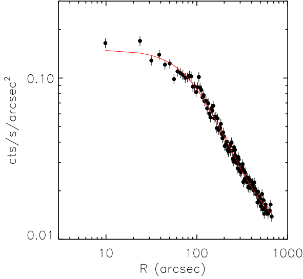
Figure 13. Surface brightness profile of the X-ray emission of A523. The best fit \beta -model is also shown in red.
