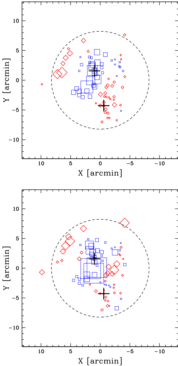
Figure 7. Dressler & Schectman bubble-plot for the \Delta -test based on local mean velocities estimated on N_{\text{nn}} + 1 galaxies. Spatial distribution of the 80 cluster members, each marked by a symbol: the larger the symbol, the larger is the deviation of the local mean velocity from the global mean velocity with scale \propto \exp(|\delta_{iV}|) . Thin blue squares and thick red rotated squares show where the local value is smaller or larger than the global value. The plot is centred on the cluster center and the circle (dashed line) contains the region within a radius equal to 8' \sim 0.92 h_{70}^{-1} \text{ Mpc} . Upper and lower panels refer to the cases N_{\text{nn}} = 10 and N_{\text{nn}} = 5 , respectively.
