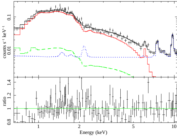
Figure 15. Upper panel: X-ray spectrum of the source taken from a 337\ h_{70}^{-1} kpc aperture. The ACIS-I data are shown in black together with the best fit model with the cluster component in red (solid line), the particle background in blu (dotted line) and the sky background in green (dashed line). Lower panel: the ratio of the data over the model is also shown.
