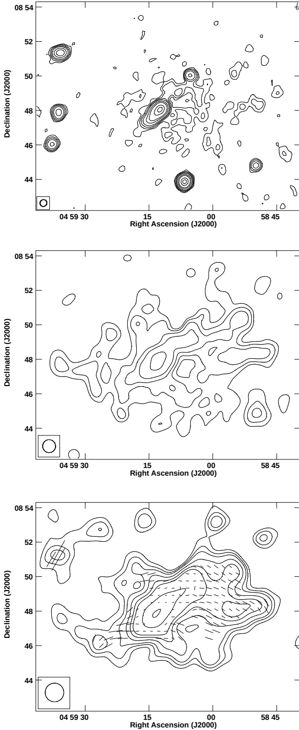
Figure 17. Top panel: total intensity contours at 1.4 GHz with a FWHM of 24.4'' \times 23.2'' (PA = -42^\circ ). The contour levels are drawn at: 0.025, 0.05, 0.1, 0.2, 0.5, 1, 3, 5 mJy/beam. The sensitivity ( 1\sigma ) is 0.012 mJy/beam. Middle panel: total intensity contours at 1.4 GHz with a FWHM of 45'' \times 45'' . The contour levels are drawn at: 0.2, 0.5, 1, 2, 5, 10 mJy/beam. The sensitivity ( 1\sigma ) is 0.07 mJy/beam. Bottom panel: total intensity contours and polarization vectors at 1.4 GHz with a FWHM of 65'' \times 65'' . The contour levels are drawn at: 0.2, 0.4, 0.6, 1, 1.5, 2, 4, 6 mJy/beam. The sensitivity ( 1\sigma ) is 0.1 mJy/beam. The lines give the orientation of the electric vector position angle (E-field) and are proportional in length to the FPOL ( 1'' \simeq 1.25\% ). In all the panels, the FOW of the image is \sim 1.8 \times 1.4 h_{70}^{-1} Mpc. MNRAS 000 , 1–21 (2015)
