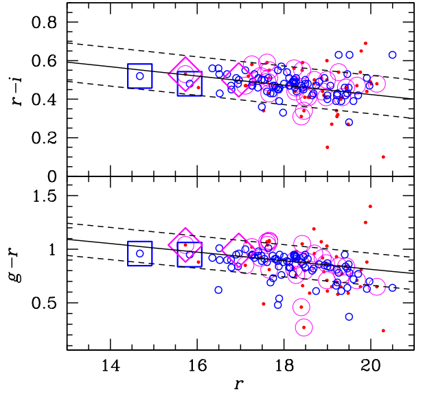
Figure 10. Upper and lower panels: r-i versus r and g-r versus r diagrams, respectively. Galaxies with available spectroscopy are shown by blue open circles (cluster members) and small red dots (field members). Very large, blue open squares indicate BCG1 and BCG2. In both panels the solid line gives the best-fit CMR as determined on spectroscopic cluster members; the dashed lines define the regions within which photometric cluster members are selected. To stress the problem of contamination in A523 due to the background field, we indicate galaxies belonging to the BACKstruct with large magenta open circles. Very large, magenta open rotated squares indicate WBgal and EBgal, the second one not included in our spectroscopic catalogue.
