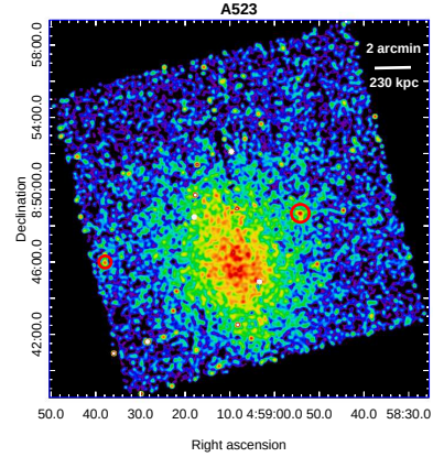
Figure 12. Chandra image in the 0.5–7 keV energy band smoothed on a 10'' scale. The image was divided by the exposure map at 1.4 keV to correct for exposure variations. The detected point sources connected with galaxies belonging to the background groups are highlighted by two red open circles.
