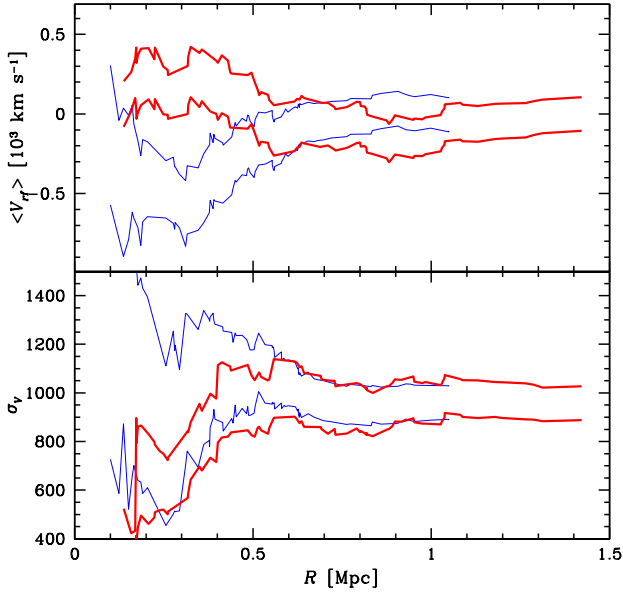
Figure 9. Error bands of mean velocity and velocity dispersion profiles computed as in middle and bottom panels of Fig. 5. Thin blue lines refer to BCG1 as center and thick red lines refer to BCG2 as center. The comparison highlights the difference in mean velocity between populations surrounding the two BCGs.
