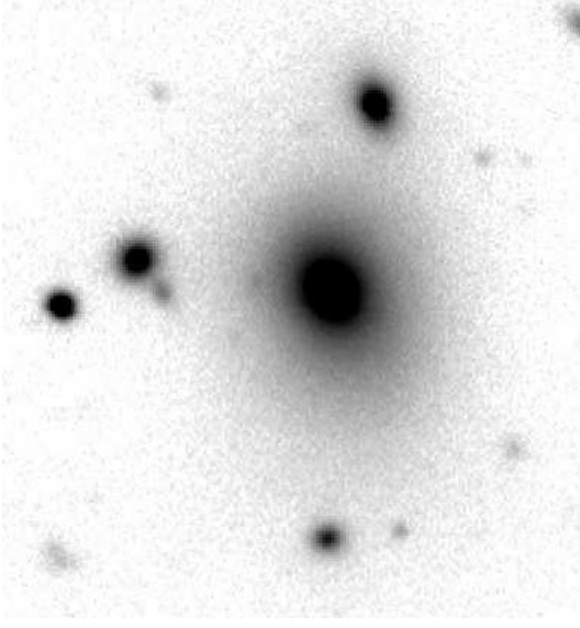
Figure 3. Zoomed-in INT r -image to view the details of the halo of BCG1, the brightest cluster galaxy specifically related to the northern subcluster. (The FOW of the image is \sim 125 \times 130 h_{70}^{-1} kpc).
