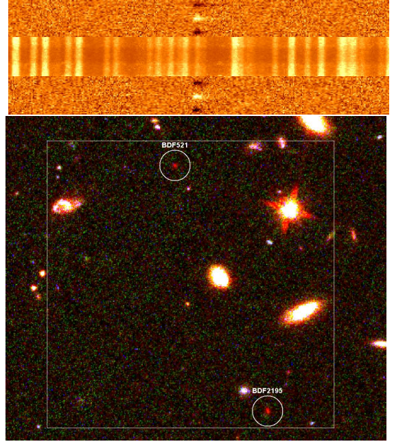
FIG. 1.— Top: the FORS2 S/N spectra of BDF521 (top) and BDF2195 (bottom) together with the reference RMS spectrum (middle). Bottom: the two objects on a HST three-color image of the BDF (blue, green and red channels are V606, I814 and Y105 respectively), the box side is of 100kpc (physical) at z=7.008 .
