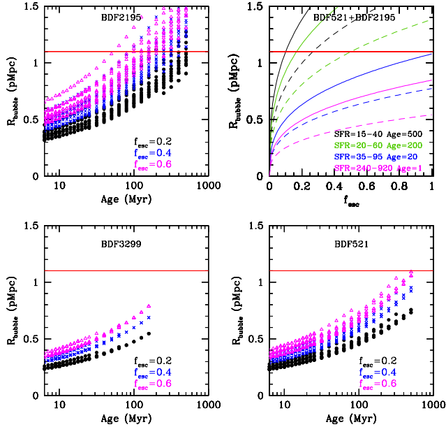
FIG. 3.— The size ( R_{bubble} ) of the ionized bubbles created by the three emitters, as a function of the age of the stellar population (bottom panels and top-left panel) for BPASSV2 SED models within 68% c.l. from the best-fit. The cases for escape fraction f_{esc}=0.2, 0.4, 0.6 are shown as black circles, blue crosses and magenta triangles respectively. Solutions having the same age and f_{esc} differ in terms of either best-fit metallicity or E(B-V), or both. The top-right panel show minimum (dashed lines) and maximum (continuous lines) R_{bubble} as a function of f_{esc} adding contribution from BDF521 and BDF2195, for stellar populations of age 500 (black), 200 (green), 20 (blue) and 1 Myr (magenta). The horizontal red line in all plots mark the minimum HII size R_{min}=1.1\text{Mpc} enabling Ly \alpha to escape.
