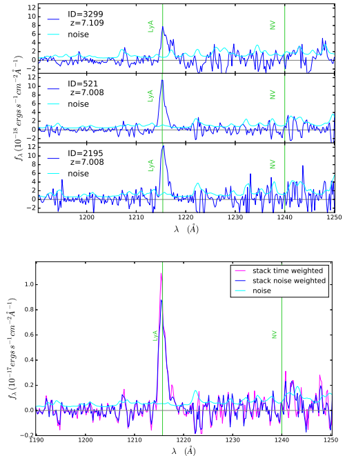
FIG. 2.— Top: the three LAE in the BDF field: BDF521 and BDF3299 from Vanzella+11 (combining old and new FORS2 data), and the new one, BDF2195. Bottom: the stacked spectrum of the 3 emitters obtained by scaling them with the total integration time applying a minmax clipping (magenta line), or weighting with the noise spectra (blue line, the resulting sky noise is shown in cyan).
