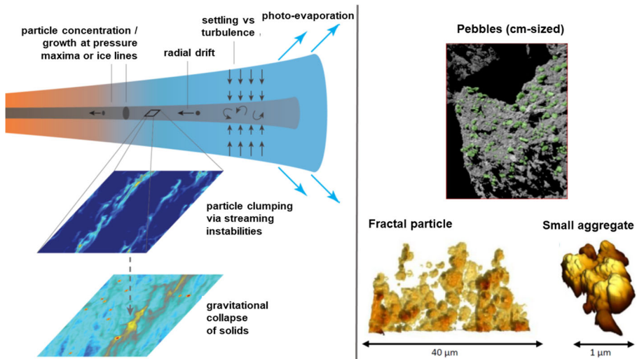
Fig. 1 Left: Processes in protoplanetary discs giving rise to gas streaming instabilities and the formation of pebbles and planetesimals [12]; Right (67P building blocks): pebbles on the surface imaged by the Comet Infrared and Visible Analyser (CIVA) onboard Philae (top) [168] and 3D rendered images obtained with the Micro-Imaging Dust Analysis System (MIDAS) (bottom) [139]
