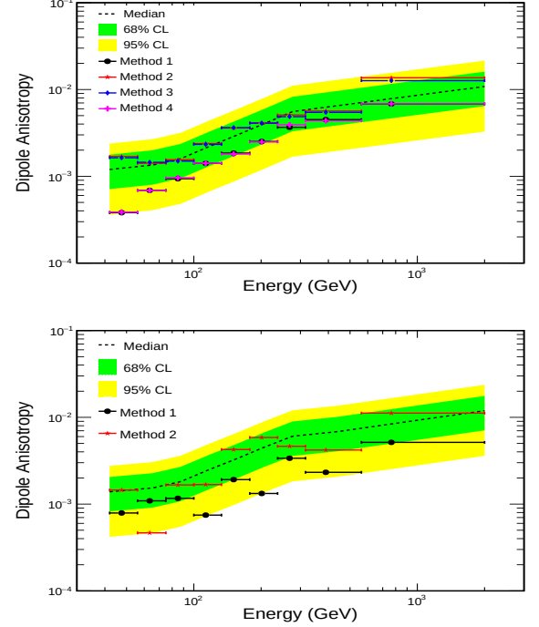
FIG. 2. Dipole anisotropies as a function of energy. Top panel: simulated isotropic data using Methods 1-4. Bottom panel: real data using Methods 1-2. The markers (median energy value calculated for a power-law flux with a spectral index of -3) show the results and the horizontal error bars indicate the energy bin width. The colored bands show the expected central confidence intervals of the white-noise at 68% and at 95%.
