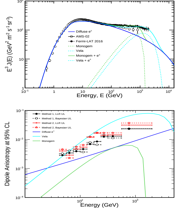
FIG. 3. Top panel: CRE spectra measured by the Fermi-LAT [6] and AMS02 [15]. Blue line: Galactic CRE evaluated with DRAGON-FLUKA [20]; Green line: Monogem alone (dashed) and total (solid). Cyan line: Vela alone (dashed) and total (solid). Bottom panel: Upper limit at 95% CL on dipole anisotropies as a function of energy. The markers in this panel show the actual measurements.
