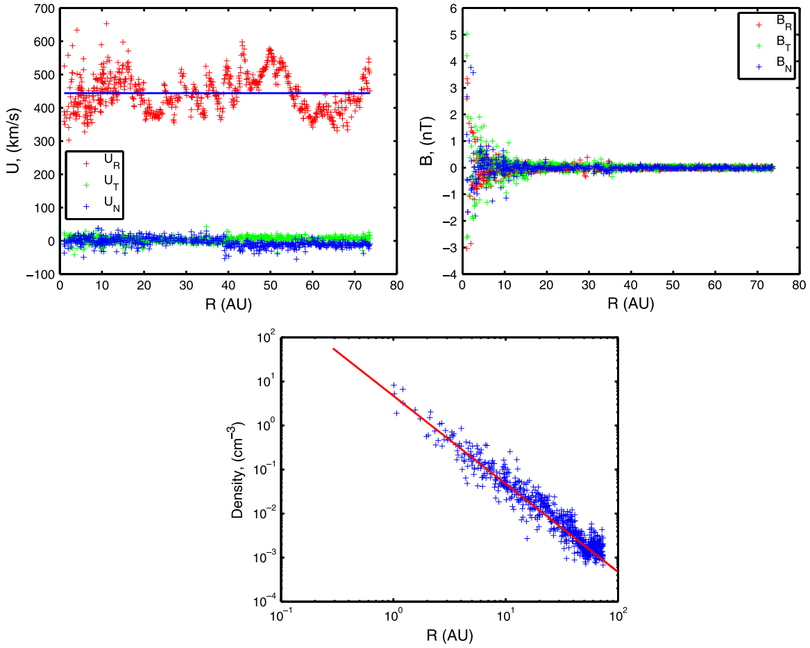
Figure 14. Top-left: solar wind velocity as a function of heliocentric distance. Top-right: magnetic field as a function of heliocentric distance. Bottom: solar wind density as a function of heliocentric distance. The red curve describes \rho = \rho_0(r_0/r)^2 , where \rho_0 is the solar wind density at r_0 ( =0.29 AU).
