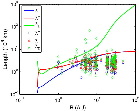
Figure 6. Comparison of the theoretical and observed correlation lengths as a function of heliocentric distance. The blue, red, and green curves correspond to the theoretical correlation lengths of forward propagating modes, backward propagating modes, and the residual energy, respectively. The blue, red, and green scatter diagrams correspond to the corresponding observed correlation lengths.
