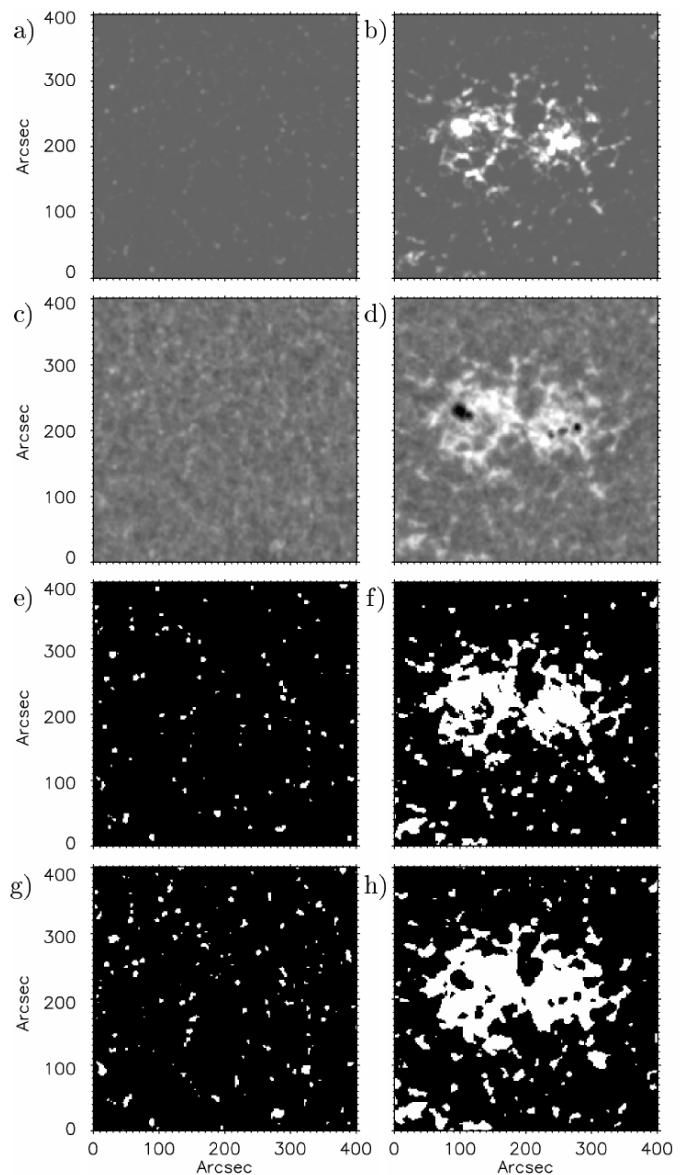
Fig. A.1. Magnified 400 \times 400 arcsec 2 sub-arrays of the images shown in Fig. 1 for a network (left) and a plage region (right). From top to bottom: (a, b)) SDO/HMI unsigned (and spatially degraded) magnetogram; (c, d)) Rome/PSPT Ca II K; the corresponding segmentation masks derived with Method 1, i.e. constant thresholds, from (e, f)) the magnetograms and (g, h)) the Ca II K images. The magnetograms are saturated in the range [-300, 300] G (the negative value was chosen merely to improve visibility of the pixels), and Ca II K observations in the range [0.5, 1.6] (the QS has the average value of 1).
