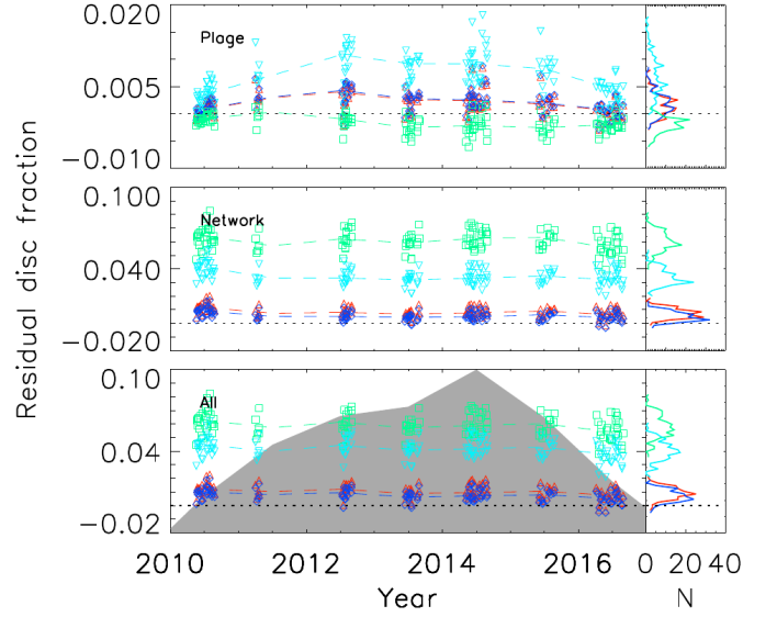
Fig. B.4. Left: Difference between the disc fraction of magnetic features derived from SDO/HMI observations with reduced spatial resolution and reconstructed magnetograms with PF* (red upward triangles), PFL* (blue rhombuses), LFL* (green squares), and PF (light blue downward triangles). Each of the upper two panels corresponds to a different feature (as marked in each panel) identified with Method 1, while the bottom panel is for all features together. The dashed lines connect annual median values, while the dotted horizontal lines are for a difference of 0. The shaded surface in the lower panel is as in Fig. 15. Right: Distribution functions of the residual disc fractions.
