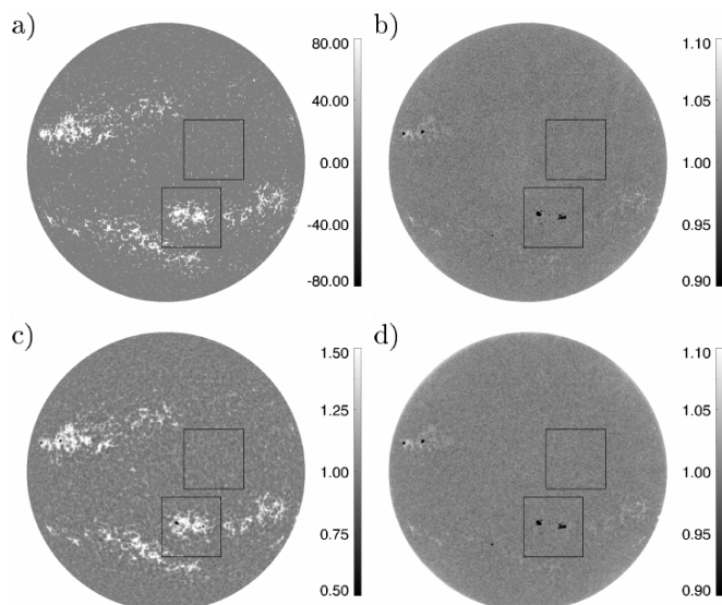
Fig. 1. Examples of the observations analysed in this study taken on 01/04/2011 at 09:06:00 UT: (a)) SDO/HMI unsigned B_{\text{LOS}} magnetogram, (b)) SDO/HMI continuum contrast image (i.e. compensated for intensity CLV), (c)) Rome/PSPT Ca II K and (d)) red continuum contrast images. The grey-scale bars on the right-hand side of each panel show magnetic signal in G and contrast, respectively. The squares indicate the insets shown in Fig. A.1.
