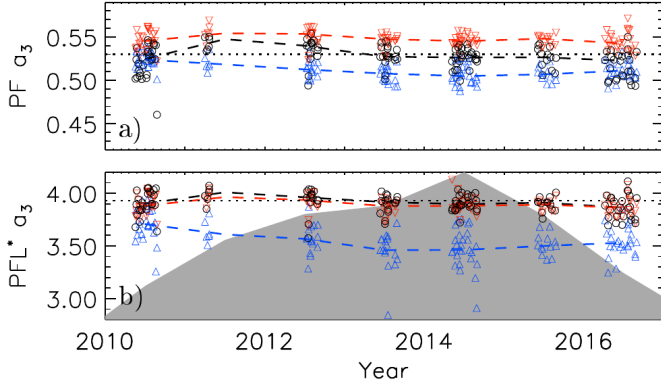
Fig. 6. Parameters of the fits (Eq. 1) as a function of time, derived for all bright features (black), as well as for the network (blue), and plage (red) separately, for PF (a) and PFL* (b) fits. The dashed lines connect the median values obtained from all analysed images within a given year, while the dotted lines mark the values of the parameters of the best fit derived in Sect. 3.1. The shaded grey surface in panel b) shows the plage areas determined with Method 1 from the Rome/PSPT images. The areas were scaled to have a maximum value of 4.2 and minimum value 2.8 in order to match the range of values shown in panel b). They indicate the level of solar activity at the considered times.
