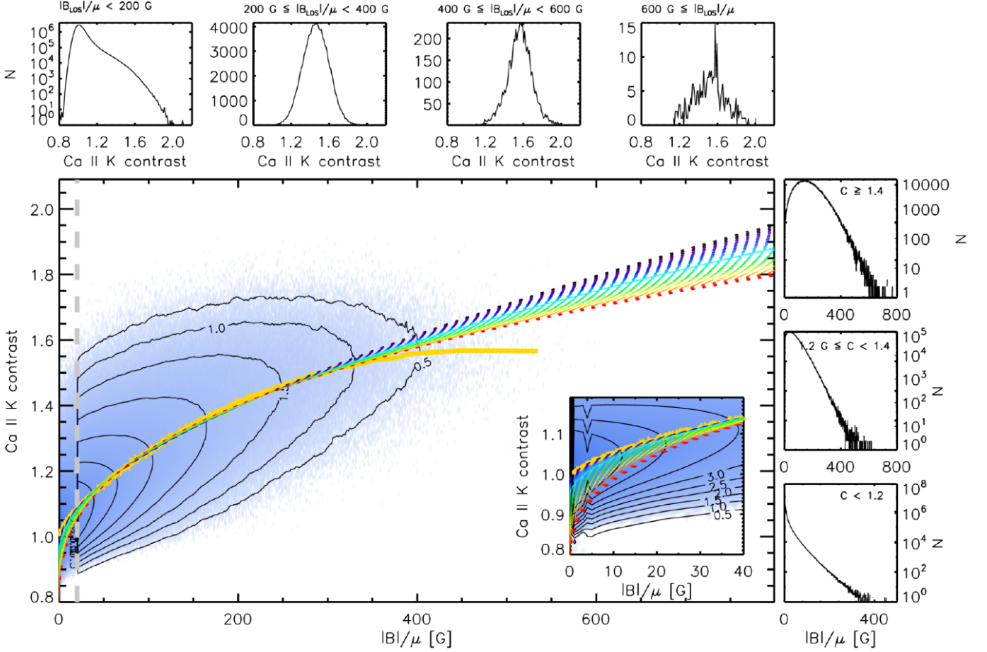
Fig. 5. Same as Fig. 3 but showing only the results of a power law function (PF) on the binned curve over |B_{\text{LOS}}|/\mu (yellow curve) by varying the |B_{\text{LOS}}|/\mu threshold, i.e., the magnetogram noise cut-off (dotted coloured curves). The threshold is 1 G for the black curve and gets to 50 G for the red curve. The curve corresponding to the 20 G threshold adopted in this study is shown with the light blue solid curve. The thick yellow curve shows 5000-point running mean over |B_{\text{LOS}}|/\mu . The vertical grey dashed line denotes the 20 G threshold in |B_{\text{LOS}}|/\mu .
