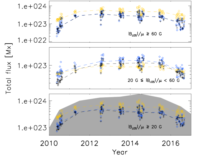
Fig. 16. Total unsigned magnetic flux in Mx of AR derived from the magnetograms (yellow circles for the original and black plus signs for the reduced spatial resolution ones) and from the unsigned magnetograms reconstructed from Ca II K observations with PFL* (blue rhombuses). Each of the upper two panels corresponds to a different type of features (as listed in the panels) identified with Method 1, while the bottom panel is for all features together. The dashed lines connect the annual median values. The shaded surface in the lower panel is as in Fig. 15.
