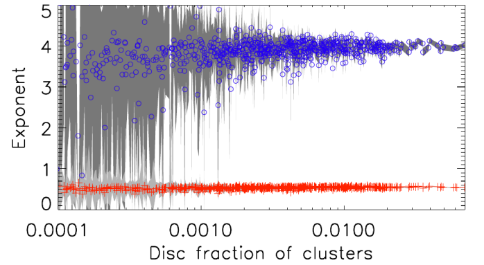
Fig. 9. Exponents of the PF (red) and PFL* (blue) fits as a function of size for individual activity clusters. The light grey and dark grey shaded areas denote the 1\sigma error in the fit parameters for PF and PFL*, respectively.
