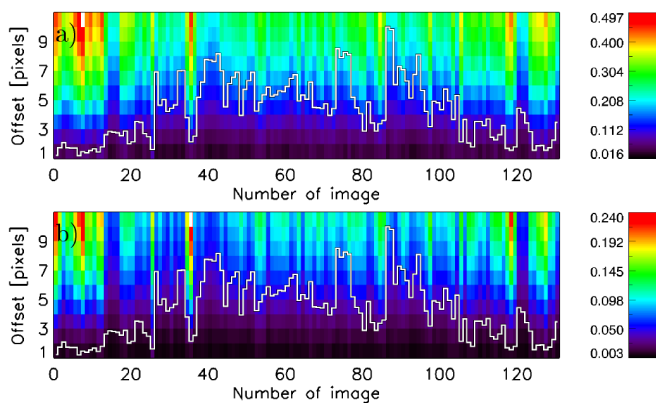
Fig. 10. Colour-coded relative errors in the exponent derived with PF (a) and PFL* (b) due to misalignment of the analysed images. Each Ca II K image was randomly shifted in both x and y directions by up to 10 pixels. The boxes give the average error after 1000 realisations. The y axis gives the value of the maximum possible offset in any direction. The x axis indicates the analysed images ordered by date covering the period 2010–2016. Colour bars show the relative errors in the computed exponents. Over-plotted with white are the plage areas derived from the Ca II K images. The areas were scaled in the range [0,9] and are shown to indicate the activity level.
