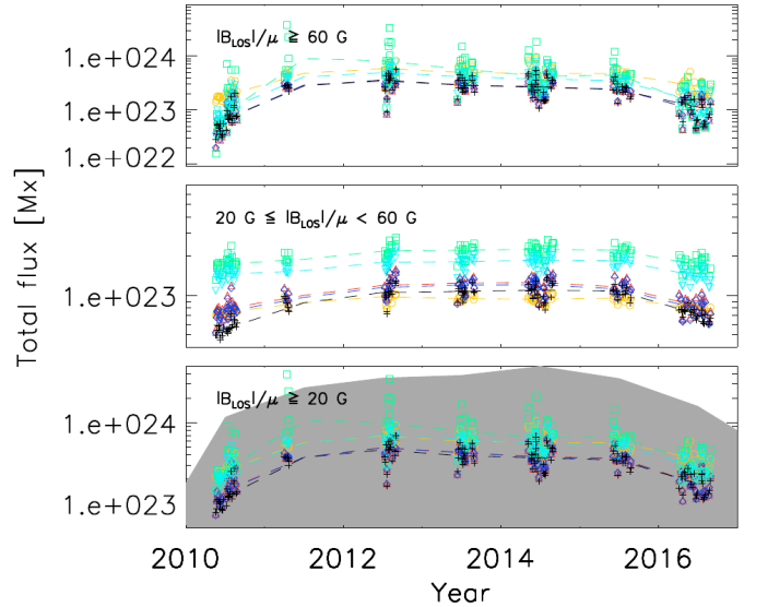
Fig. B.5. Total unsigned magnetic flux in Mx of AR derived from the magnetograms (yellow circles for the original and black plus signs for the reduced spatial resolution ones) and from the unsigned magnetograms reconstructed from Ca II K observations with PF* (red upward triangles), PFL* (blue rhombuses), LFL* (green squares), and PF (light blue downward triangles). Each of the upper two panels corresponds to a different type of features (as listed in the panels) identified with Method 1, while the bottom panel is for all features together. The dashed lines connect the annual median values. The shaded surface in the lower panel is as in Fig. 15.
