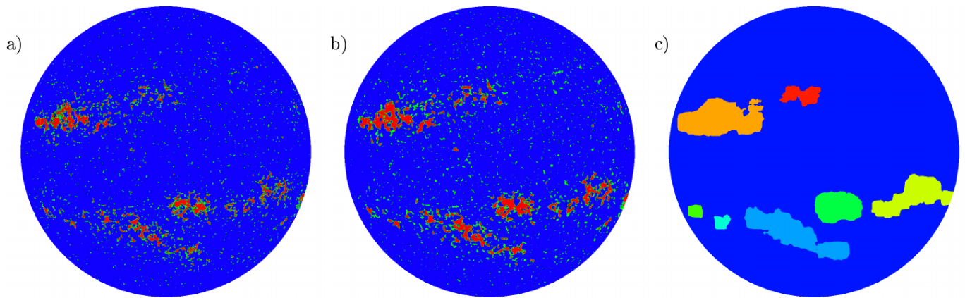
Fig. 2. Segmentation masks of bright magnetic features derived from the observations shown in Fig. 1 by applying the 2 methods described in Sect. 2.3. (a)) Mask of magnetogram and (b)) Ca II K image derived with Method 1, showing plage (red), network (green), and QS (blue). (c)) Mask of magnetogram derived with Method 2, showing individual activity clusters with different colours (the QS is in dark blue). The masks are shown prior to the exclusion of the sunspot regions.
