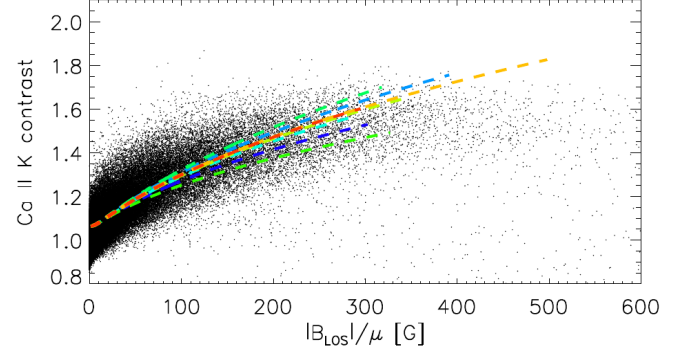
Fig. 8. Ca II K contrast plotted against |B_{\text{LOS}}|/\mu for all activity clusters identified with Method 2 in observations shown in Fig. 1 (black dots). The coloured curves are the result of the PFL* fit to the individual clusters, shown with the same colours as in Fig. 2c).
