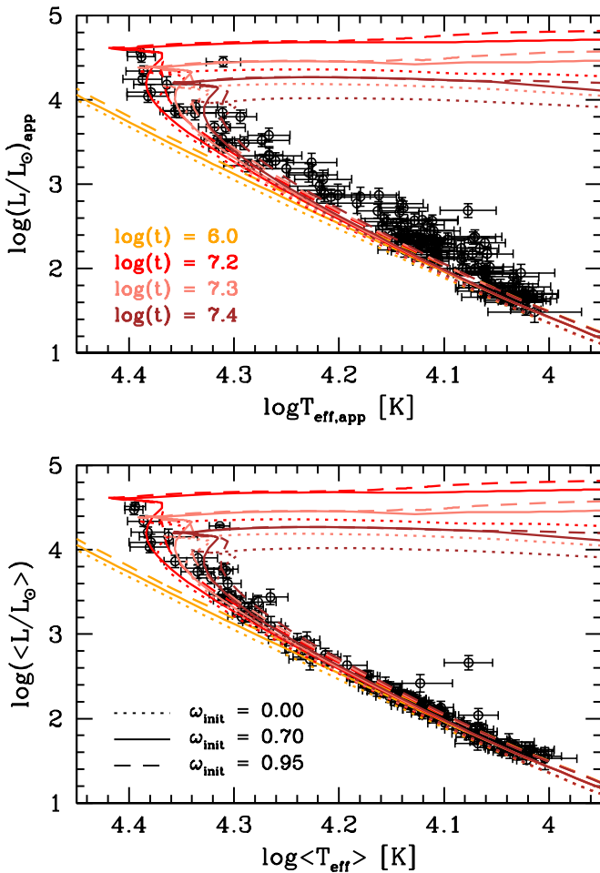
Fig. 8. HR diagrams using apparent ( top panel ) and averaged over the stellar surface ( bottom panel ) stellar parameters. Isochrones for various ages and initial rotation rates are overlaid (Georgy et al. 2013).
