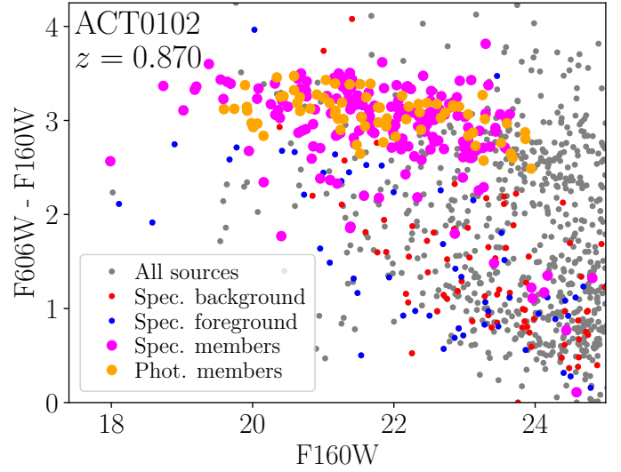
Fig. 6. Colour magnitude diagram of ACT0102. Spectroscopic members are shown in magenta and photometrically selected ones in orange (see Sect. 3 for more details on our selection criteria). Spectroscopically confirmed background and foreground objects are indicated by red and blue dots, respectively.
