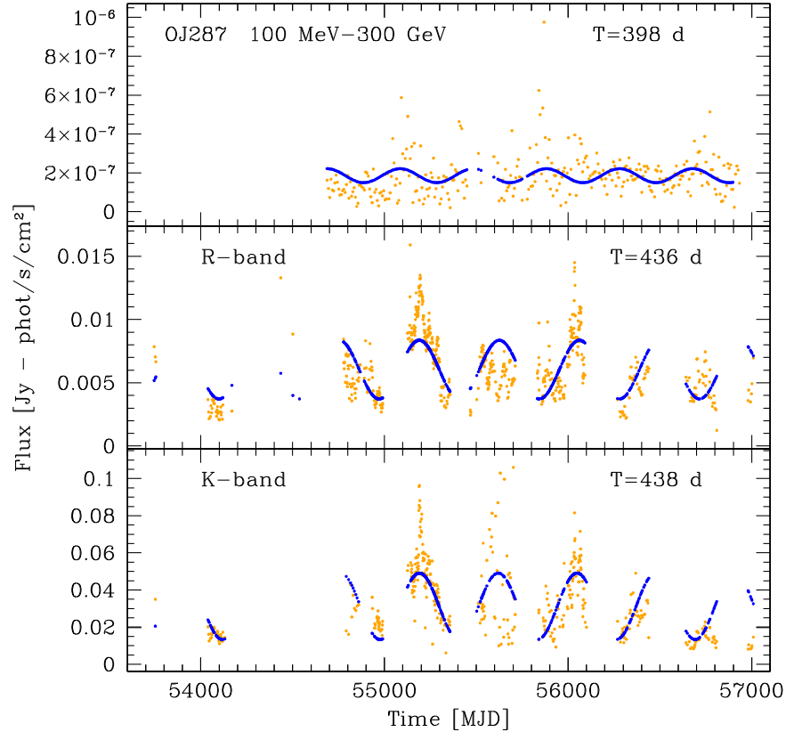
Figure 3. Same as Figure 2 for OJ 287. The amplitudes of the sinusoidal curves are A = 3.60 \cdot 10^{-8} photons \text{s}^{-1} \text{cm}^2 in 100 MeV–300 GeV ( T = 398 days), A = 0.0023 Jy in R ( T = 436 days), and A = 0.0179 Jy in the K band ( T = 438 days).
