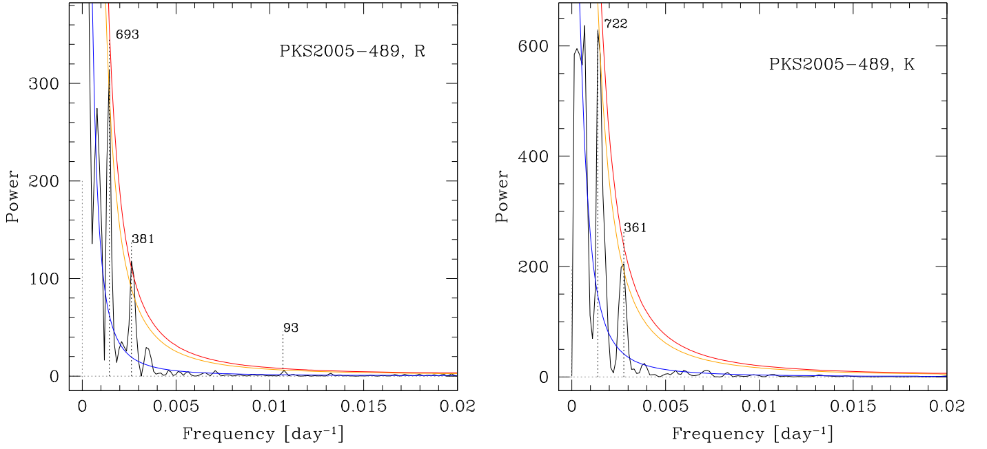
Figure 11. The same as Figure 7 for PKS 2005-489.
