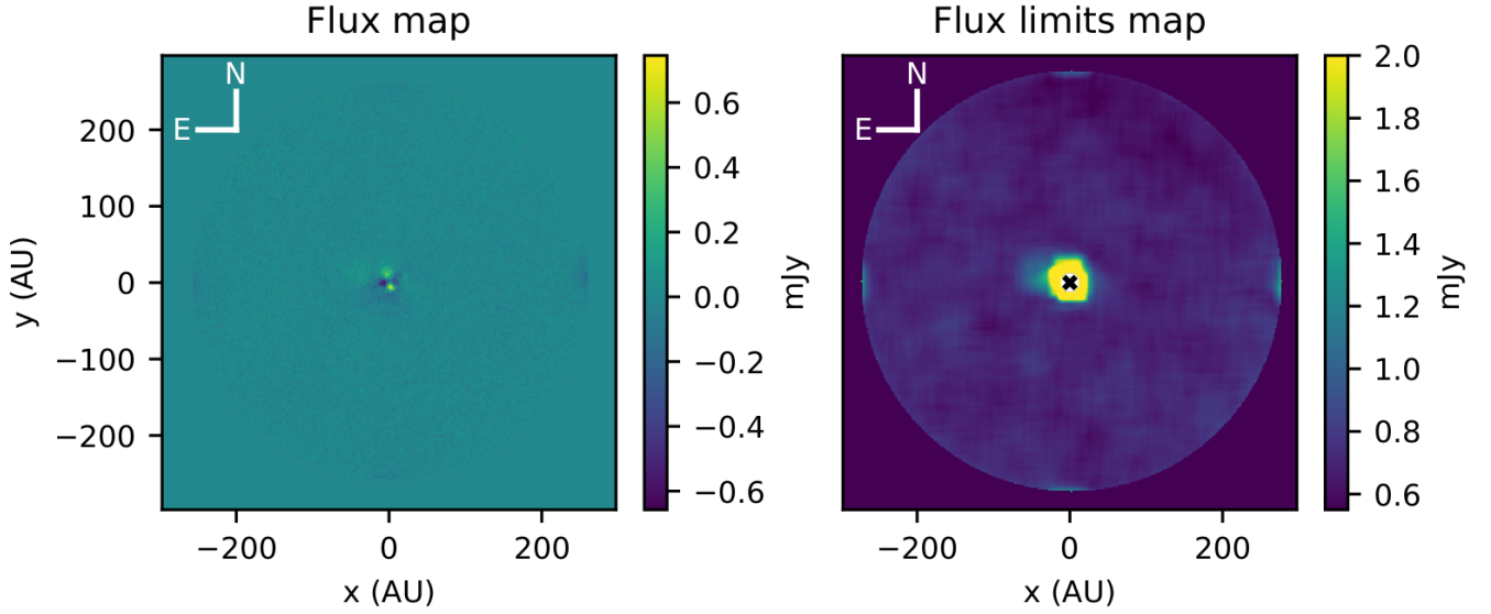
Figure 2. Left: Reduced master image of HR 8799, centered on the star. The planets are not visible in the reduced data. Positive and negative structures are visible in the center from imperfect subtraction of the stellar PSF. Right: 5\sigma flux limit map. The center of the image around the star where the limits are highest has been occulted for clarity. The decrease of the limits with radius shows that stellar features dominate the inner 40 AU, and further out a background sensitivity is achieved.
