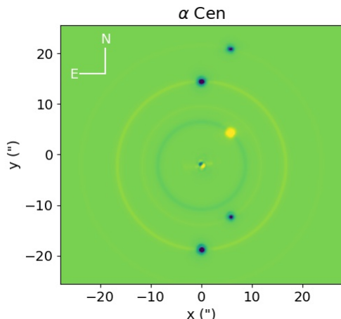
Figure 1. Example of circularised PSF subtraction for the binary stars of \alpha Cen. \alpha Cen A is the central source and \alpha Cen B the companion. The central source is subtracted, while the subtraction of the circularised PSF results in a dark ring at the separation of the second source. The second source is still clearly visible, as are in this case the chop/nod shadows of both sources and their corresponding bright rings.
