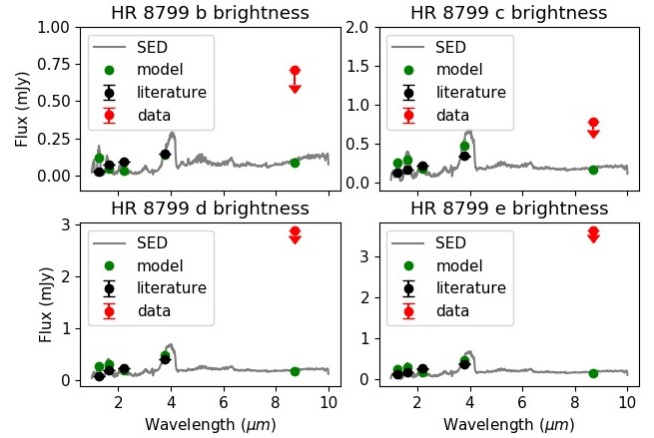
Figure 4. Theoretical spectral energy distributions (SED, grey) for HR 8799 bcd from top left to bottom right using the BT SETTL model with temperatures and surface gravities from Marois et al. (2008, 2010) . The flux density values of the earlier measurements are marked in black and the values derived from the model are marked in green. The 5\sigma upper limits calculated in this work are marked in red. All four planets have expected J8.9 flux densities below the derived limits, resulting in a nondetection of the planets in the data.
