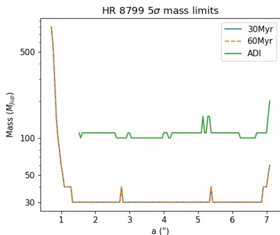
Figure 5. Upper mass limits ( 5\sigma ) for the mass of any objects in the HR 8799 system as a function of separation from the star. At small separations the flux from stellar residuals causes high mass limits, but at 1" (40 AU) these become negligible and the background dominates for the circularised PSF subtracted data. The mass limit levels out to 30 M_{\text{Jup}} , as indicated by the black dotted line. The increase furthest out is due to the chop/nod shadows located at 8". The mass limits resulting from data reduced with traditional ADI beyond 1.5" are shown in green and are around 100 M_{\text{Jup}} .
