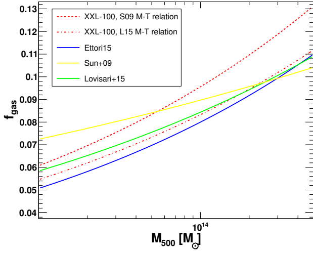
Fig. E.1. Gas fraction curves for the XXL-100-GC sample estimated assuming the hydrostatic M - T relations of Sun et al. (2009 , dotted red curve) and Lovisari et al. (2015 , dash-dotted red curve), compared to literature measurements based on hydrostatic masses.
