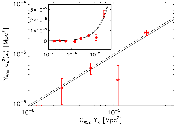
Fig. 9. Planck SZ flux Y_{500} d_A^2(z) versus Y_{X,500} for the XXL-100-GC sample (red diamonds). The expected value 0.924 (Eq. (19) in Arnaud et al. 2010 ) is the solid black line and the unity is shown as the dashed line. The inset presents the same data points in the lin-log plane to show also the low Y_{X,500} bins. The numerical values and error bars for the 8 points are given in Table 2.
