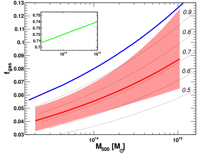
Fig. 10. f_{\text{gas}} - M relation within r_{500,\text{MT}} obtained for XXL clusters (red line) compared to Ettori (2015) , (blue). The green line in the inset shows the recovered hydrostatic bias 1 - b = \frac{M_X}{M_{\text{WL}}} required to bring the two measurements in accord. The dashed lines show the expected true gas fraction curves for constant values of 1 - b in the range [0.5–0.9].
