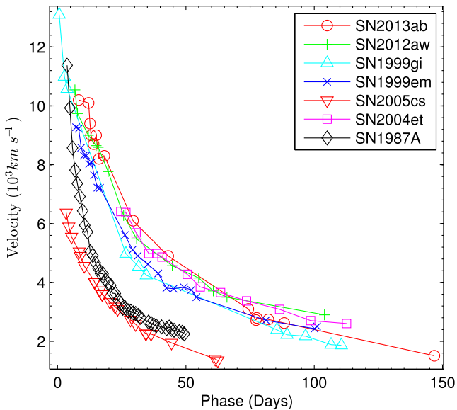
Figure 15. The evolution of photospheric velocity ( v_{ph} ) of SN 2013ab is compared with those of other well-studied SNe. The v_{ph} plotted here are the absorption trough velocities (from He\ I lines at early phases, and Fe\ II at late phases.)
