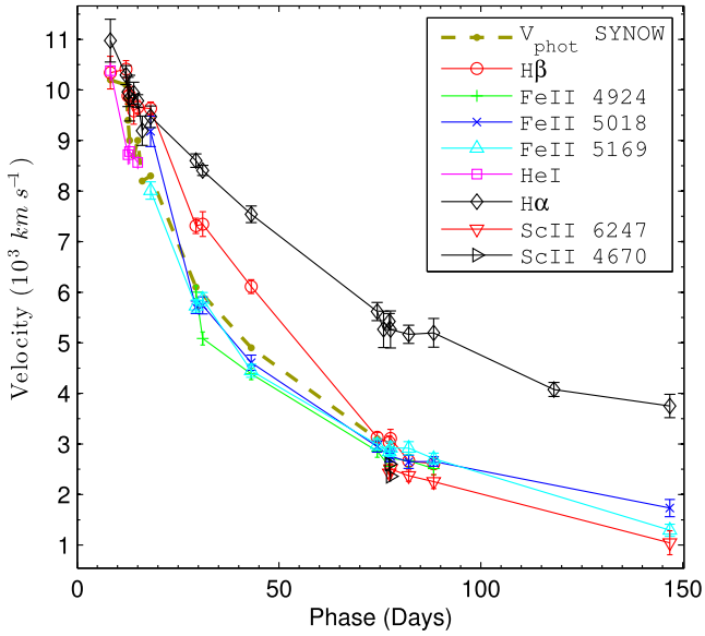
Figure 14. Evolution of the H\alpha , H\beta , He\ I , Sc\ II and Fe\ II line velocities. The velocities are estimated through the Doppler shift of the absorption minima. The expansion velocities at the photosphere ( v_{ph} ) estimated from SYNOW fits of He\ I line until 18 d and simultaneous fits for Fe\ II lines at later phases (see Table 2) are shown as a comparison.
