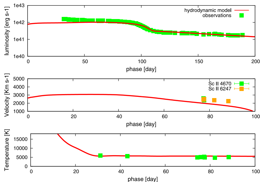
Figure 18. Comparison of the evolution of the main observables of SN 2013ab with the best-fitting model computed using the general-relativistic, radiation-hydrodynamics code (total energy 0.35 foe, initial radius 4.2 \times 10^{13} cm, envelope mass 7 M_{\odot} ). Top, middle and bottom panels show the bolometric light curve, the photospheric velocity and the photospheric temperature as a function of time. To better estimate the photosphere velocity from observations, we use the minima of the profile of the Sc II lines which are considered good tracer of the photosphere velocity in Type II SNe. As for the photospheric temperature, we use the blackbody temperature derived from the blackbody fits to the spectral continuum.
