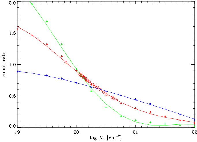
Fig. 3. ROSAT count rate corresponding to an unabsorbed flux of 10^{-11} erg cm ^{-2} s ^{-1} versus the Galactic hydrogen column density N_H for the three values of the X-ray photon spectral index \Gamma_x = 1 (blue), 2 (red), and 3 (green). Plus signs indicate the values derived with WebPIMMS, and solid curves represent polynomial fits through them. Open circles correspond to the N_H values of our LPBLs.
