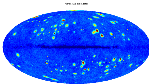
Fig. 4. Distribution on the sky of the Planck ESZ clusters (the signal has been amplified to be seen).
