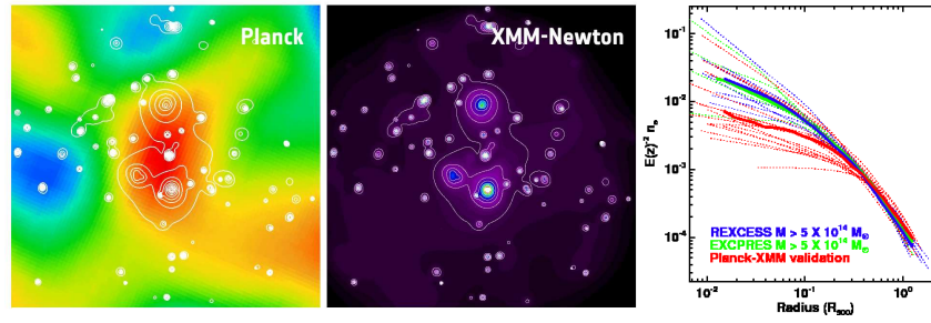
Fig. 5. Left panel: Planck SZ and XMM X-ray images of PLCKG214.6+37.0. Right panel: electronic density profiles of Planck and REXCESS clusters.
