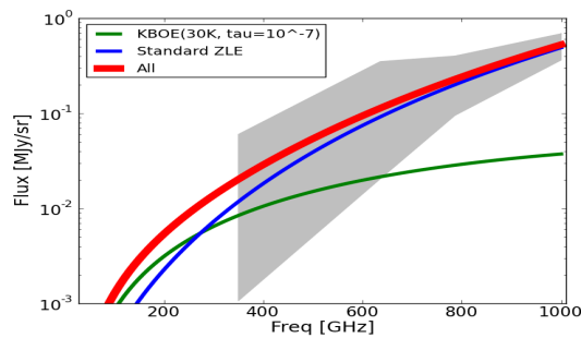
Fig. 2. The expected spectral energy distribution (SED) for the sky averaged ZLE (blue line) and an hypothetical cold dust component with T_{\text{dust}} = 30 K, \tau = 10^{-7} (green line) and their sum (red line) compared with the COBE/FIRAS spectrum (gray patch).
