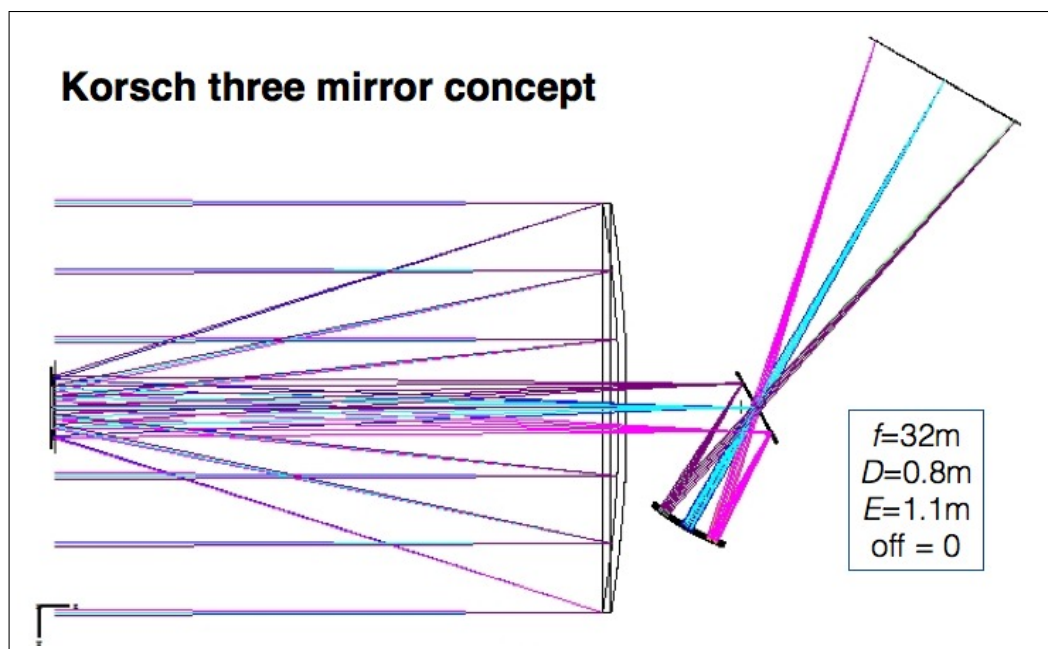
Figure 6. A possible optical lay-out of the Theia telescope. It is a three mirror anastigmat with a centered Korsch configuration s. The main parameters of this Korsch telescope is a mirror diameter of D = 0.8\text{ m} , a focal length f = 32\text{ m} , ellipticity of E = 1.1\text{ m} .
