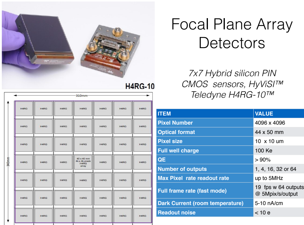
Figure 7. Top left : photograph of a Teledyne HR4G-10 HyViSI detector. Bottom left: schematical display of the focal plane with its 7 \times 7 Teledyne detectors. Right: Characteristics of the Teledyne H4RG10-HyViSI detector.
