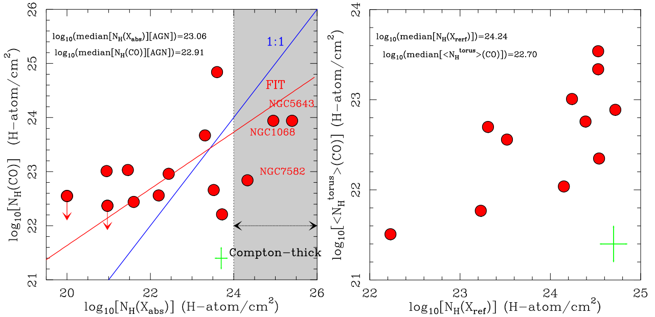
Fig. 17. Left panel: comparison of the column densities of neutral gas measured from CO toward the AGN ( N_H(\text{CO}) ; in units of H atoms per cm 2 ) with the column densities derived by modeling the absorption of X-rays ( N_H(X_{\text{abs}}) ; Ricci et al. 2017a) in the galaxies listed in Table 3 and in NGC 613. In this comparison we use the HSR datasets of ALMA for the core sample of GATOS. The blue color is used to draw the 1:1 line, while the red color identifies the linear bisector fit to the data. Right panel: comparison of the average surface density of molecular gas measured for the molecular tori of the galaxies listed in Table 3 ( \langle N_H^{\text{torus}} \rangle (\text{CO}) , in units of H atoms per cm 2 ) with the corresponding column density derived in Sect. 7.2 by modeling the reflection of hard X-rays ( N_H(X_{\text{ref}}) ). Errorbars at the lower right corners in both panels account for the total uncertainties on the molecular gas mass estimates due to the assumed conversion factors ( \sim \pm 0.2 dex), and for a \pm 0.15 dex uncertainty on the gas column densities derived from the modeling of X-rays.
