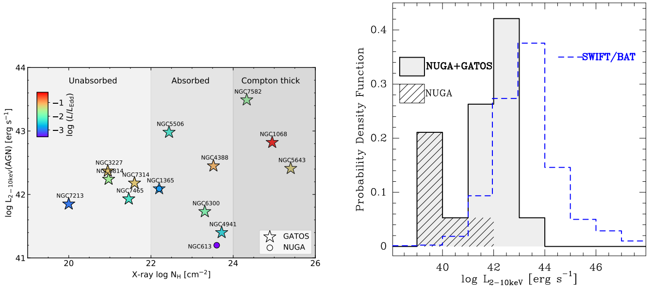
Fig. 1. Left panel: comparison of the distribution of intrinsic AGN luminosities measured in the 2–10 keV X-ray band (corrected for absorption) and the column densities, N_H , derived from hard X-rays, as measured by Swift /BAT in the 14–150 keV band for the combined GATOS sample listed in Table 1 (star markers) (Ricci et al. 2017a). We also include the data of NGC 613 from the NUGA sample (Combes et al. 2019) (circle), which also has NGC 1365 as a target in common with GATOS. Symbols are color-coded to reflect the Eddington ratios estimated by Koss et al. (2017). Right panel: comparison of the probability density function (PDF) of AGN luminosities in the 2–10 keV band for the combined sample of GATOS and NUGA (gray-filled histogram) and the Swift /BAT sample of Ricci et al. (2017a) (blue histogram). We identify the distribution of NUGA targets by the hatched area. This figure illustrates the complementarity of NUGA and GATOS samples in covering a significant ( \sim 4.5 dex) range of intrinsic AGN luminosities with the combined sample of 19 nearby Seyferts used in this work.
