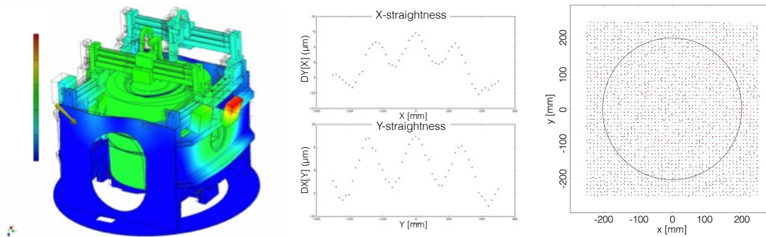
Figure 2 Flexure modelling, characterisation and correction. The FEA model was used to generate a simulation of a measured reference grid with the required shifts, shear, rotation and flexure. These terms were then evaluated from the ‘measured’ grid including removing the axis straightness and flexure. The resulting transformation was then applied to the original measurements and compared to the input reference grid. The resulting residuals were typically 3.1\mu\text{m} rms, with no remaining systematic structure.
