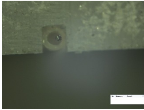
Figure 11 Retention of 120µm fibre in 0.5mm PEEK tube by pressing it into an accurately machined square groove.
