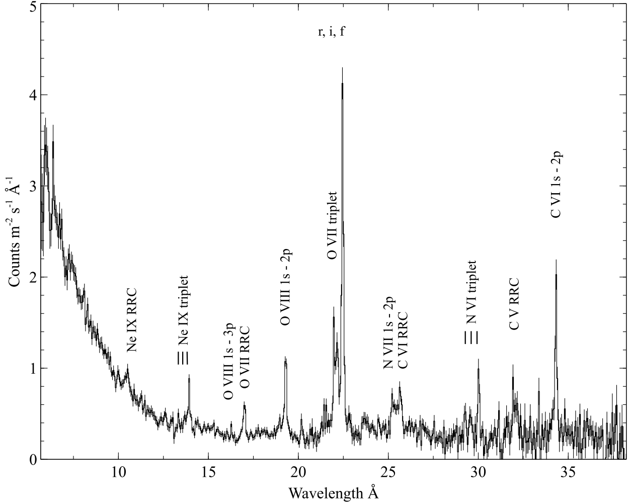
Fig. 1. The 2013–14 770 ks stacked RGS spectrum of NGC 5548 (observed frame). The strongest emission lines are labelled. The data points are shown in black. The data have been binned by a factor of two for clarity.
