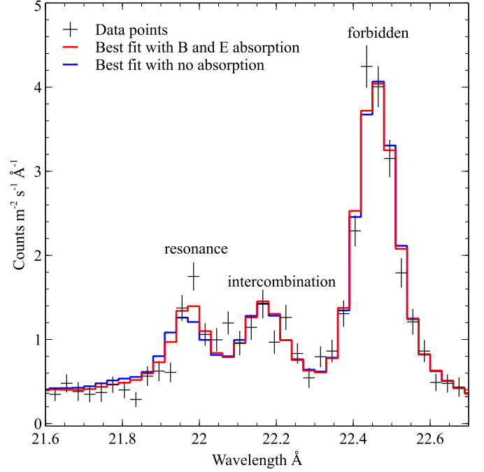
Fig. 4. Best fit model to O VII triplet. The data are shown in black. Shown in red is the best fit including absorption from X-ray WA components B and E (C-statistic = 82, for 43 d.o.f.). Shown in blue is the best fit with no absorption (C-statistic = 104, for 43 d.o.f.). In both models the outflow velocities and line widths of all three triplet lines are coupled together. The outflow velocity, line width and normalisations were left free to vary to find the best fit for each scenario.
