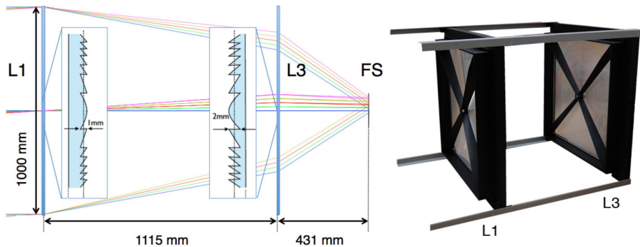
Fig. 4 Left : ray tracing diagram for the EUSO-Balloon optics with the Fresnel Lenses L1 and L3, and the focal surface; the incident rays are at off-axis angles ranging from 0° (blue) to 1° (green), 2° (red) 3° (yellow) and 4° (purple); inserts show partial sectional views of L1 and L3; right : Optical bench with Fresnel lenses L1 and L3 (8 mm thick PMMA, surface of 1 m × 1 m) mounted onto their fiberglass frames and spiders, and held at a distance of 1.11 m by an optical “sled”
