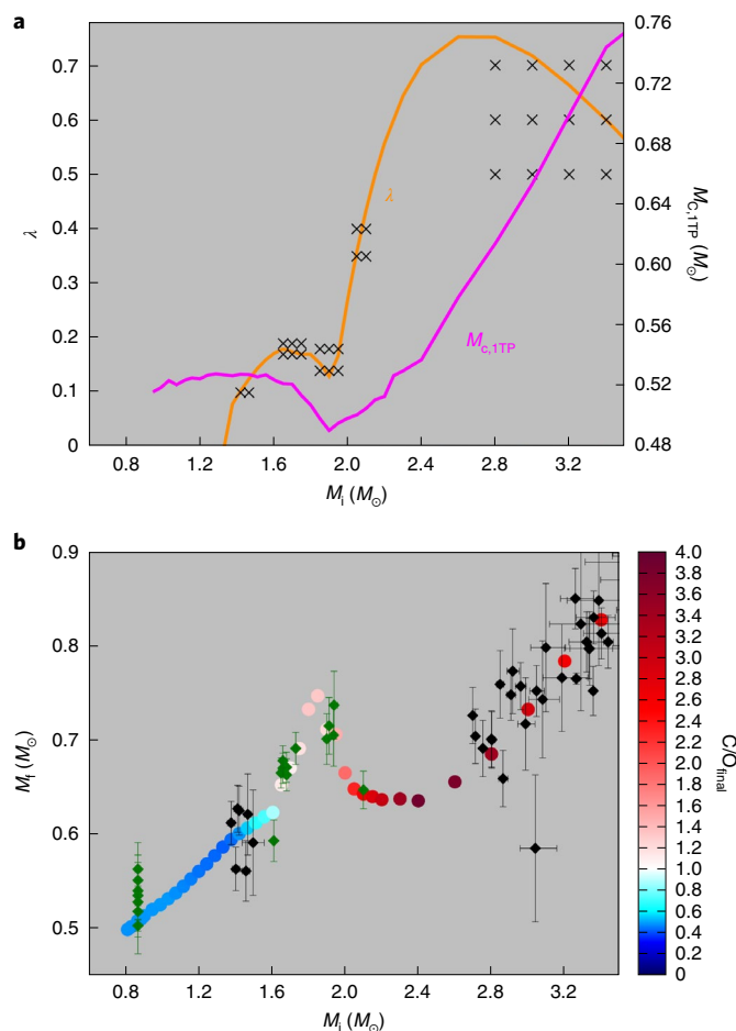
Fig. 4 | Calibration of the 3DU efficiency and the resulting theoretical IFMR. a, The values of the average \lambda (black crosses) that recover the semi-empirical IFMR data and a proposed best-fit curve for \lambda (orange line) as a function of the initial mass; the core mass at the first TP (magenta line). b, The theoretical IFMR obtained with the calibrated \lambda relation, colour-coded as a function of the final C/O (colour bar). The underlying semi-empirical IFMR (diamonds with errors bars) is the same as in Fig. 1, with the 7 newly discovered and 12 newly analysed WDs shown in green. Error bars cover a range of \pm 1\sigma (see Table 1).
