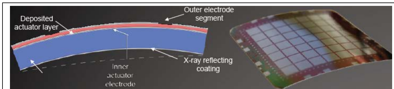
Figure 1. Left: schematic of adjustable optics segment: an X-ray reflective coating is applied to the inner convex side of the glass segment and the piezoelectric material is applied to the outer side. Right: photograph of a test segment which shows the pixellated piezoelectric material on the backside of the segment,
