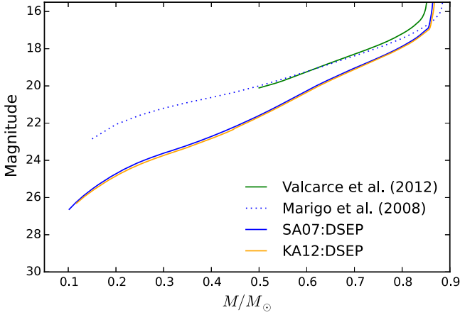
Figure 6. MLR based on the DSEP, PGPUC (Valcarce et al. 2012), and Padova (Marigo et al. 2008; Girardi et al. 2010) models for both the VMC's Y-band magnitudes and the HST F606W filter. The blue and orange curves are the DSEP MLRs for the HST data, while the green curve represents the PGPUC model for the VMC data. The dotted line is the Padova model pertaining to the VMC data, shown for comparison.
