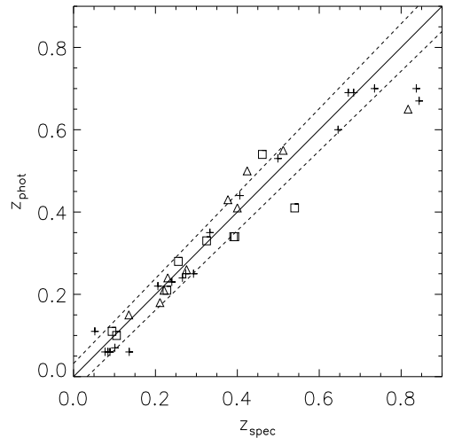
Fig. 5. Comparison between photometric estimates and spectroscopic redshifts. The continuum line represents the 1:1 relation and dashed lines show the photometric redshift error \delta z / (1 + z) = 0.03 when comparing clusters with z < 0.75 . Symbols used are as in Fig. 3.
