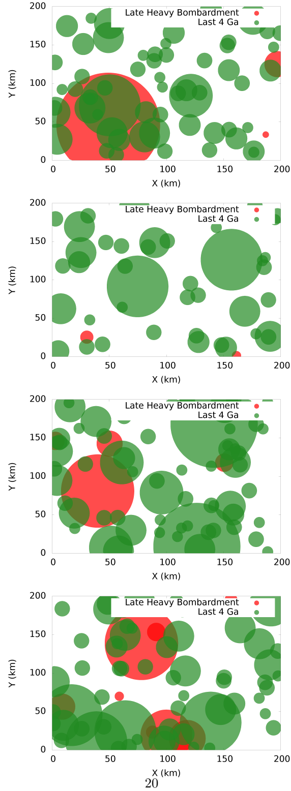
Figure 4: Four examples of crater population due produced by the LHB and by the last 4 Ga on a surface of 200 \times 200 km of Vesta.
