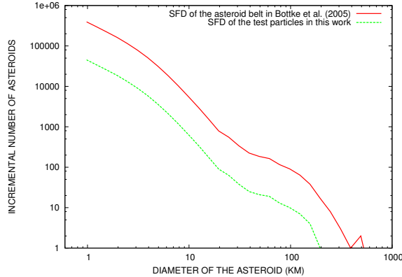
Figure 1: In red the main-belt asteroid size distribution reported in Bottke et al. (2005). In green the size distribution of the massless bodies used in our simulations.
