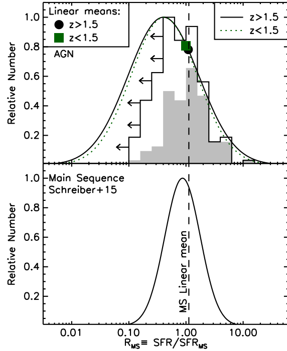
Figure 3. R_{\text{MS}} distributions for our high- z and low- z samples of X-ray selected AGNs (Top) and MS galaxies (Bottom; from S15). Here, we show the log-normal distributions with best fitting parameters shown in Table 1 (solid and dotted curves; see key). The histograms in the top panel shows the relative numbers of AGNs from our combined (i.e., low- z +high- z ) sample in each R_{\text{MS}} bin; the solid grey histogram represents those AGNs detected at > 3\sigma with either Herschel or ALMA, whereas the empty histogram (with left-pointing arrows) also includes upper limits. The solid points in the top panel indicate the linear means of the log-normal distributions (equivalent to what would be obtained via, e.g., stacking analyses) and lie within 1\sigma of the linear mean R_{\text{MS}} of MS galaxies (vertical dashed line).
