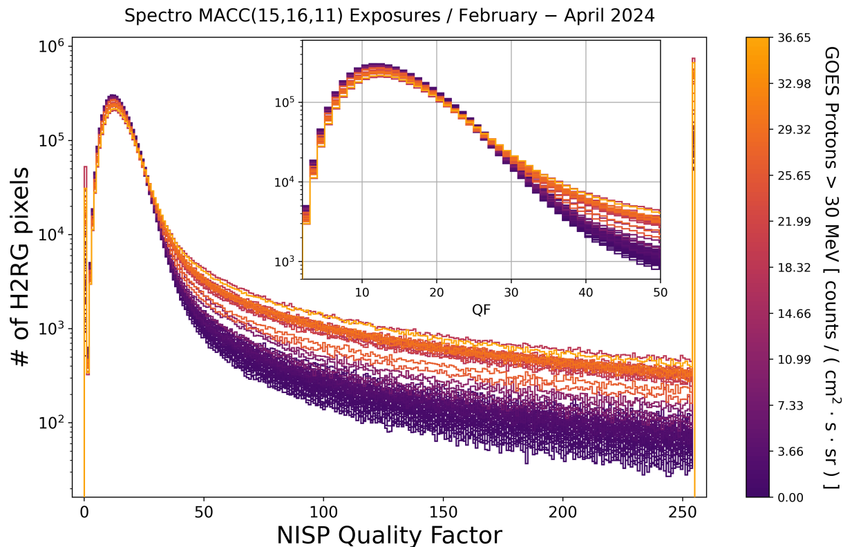
Figure 6: Example of the variations induced in the NISP QF distributions by different GOES proton flux intensities ( E > 30 MeV).
