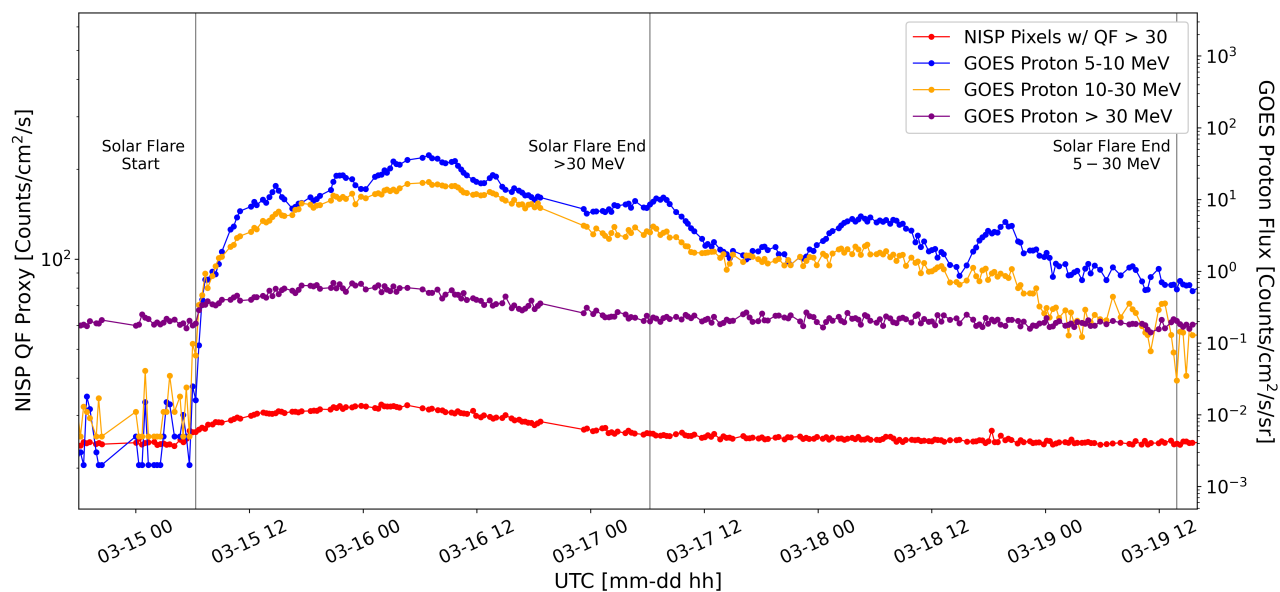
Figure 7: Comparison of the time evolution of NISP QF Proxy and GOES data during the March 2024 Solar flare. The blue, yellow, and purple data points report the Solar proton flux in different energy ranges, while the NISP measurements are reported in red. Because of the different physical units, the evolution of the NISP QF Proxy refers to the left axis, while the GOES proton flux refers to the right one.
