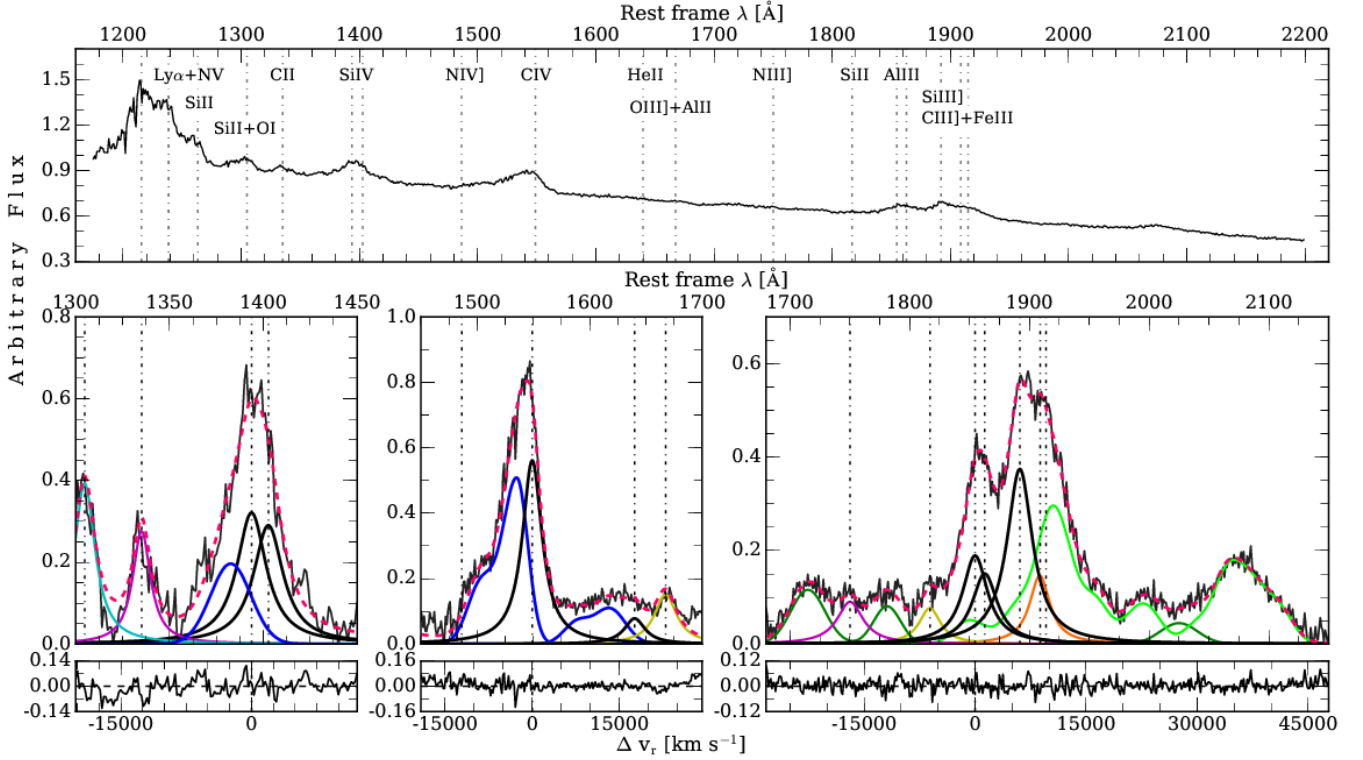
Fig. 1. Top panel: rest-frame composite spectrum (See Sect. §5.1). Abscissa corresponds to vacuum rest-frame wavelength in Å, while ordinate is in arbitrary intensity. Dot-dashed vertical lines identify the position at rest-frame of the strongest emission lines. Bottom panels: multicomponent fits after continuum subtraction for the 1400Å blend, Civλ1549 and 1900Å blend spectral regions (Sect. §4.2). In all the panels continuous black line marks the broad component at rest-frame associated to Siivλ1397, Civλ1549, Alivλ1860 and Simλ1892 respectively, while the blue one corresponds to the blueshifted component associated to each emission. Dashed pink line marks the fit to the whole spectrum. Dot-dashed vertical lines correspond to the rest-frame wavelength of each emission line. In the Siivλ1397 spectral range, the cyan line marks the contribution of Oiλ1304+Simλ1306 blend, while the magenta line corresponds to the Ciiλ1335 emission line. In the Civλ1549 region, the yellow one corresponds to the Oiiiλ1663 + Alivλ1670 blend. In the 1900Å blend range, Feii and Feii contributions are traced by dark and pale green lines respectively, magenta line marks the Niiiλ1750 and the yellow one corresponds to the Siivλ1816. Lower panels correspond to the residuals, abscissa is in radial velocity units km s -1 .
