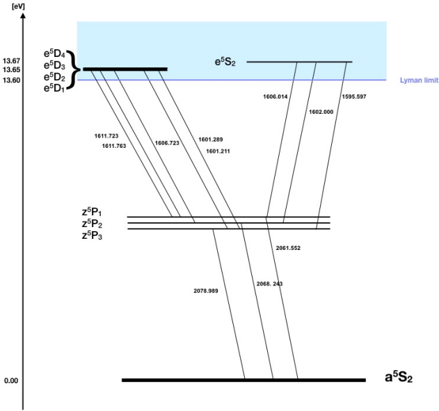
Fig. C.1. Partial Grotrian diagram showing the energy levels and the spectroscopic terms associated with the emission of FeII multiplet #48, #118 (top left) and #119 (top right). Energy level separation is not drawn to scale for clarity.
