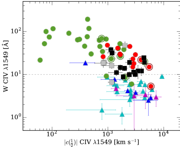
Fig. 10. Relation between rest-frame equivalent width of C IV \lambda 1549 and c(\frac{1}{2}) in km s ^{-1} . Black squares: GTC-xA. Gray squares: BAL GTC-xA. Blue triangles: Plotkin et al. (2015), magenta: Wu et al. (2012) and cyan: Luo et al. (2015). Red and green circles correspond to the Pop. A samples from S17 and FOS-A sample, respectively. Circled symbols correspond to FOS-xA and S17-xA.
