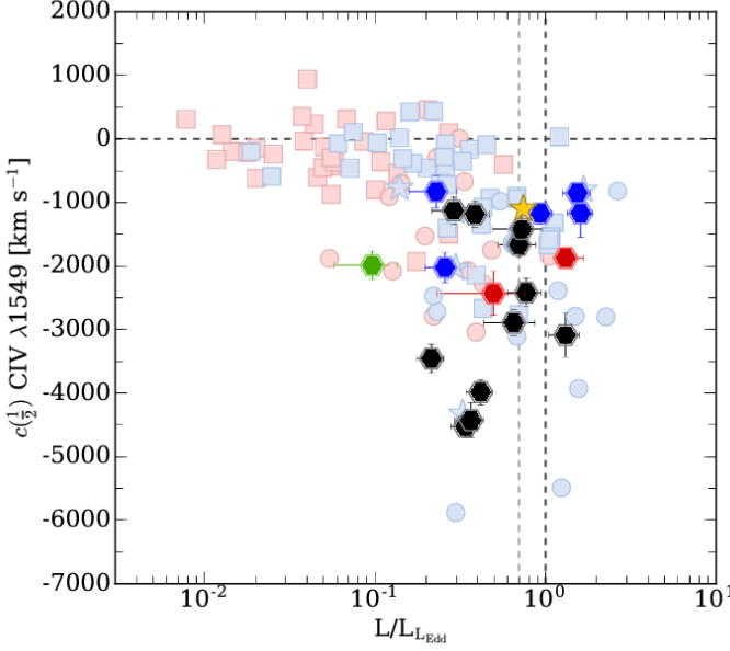
Fig. 9. Behavior of the centroid at 1/2 of total C IV \lambda 1549 profile as a function of Eddington ratio. Hexagons represent the GTC-xA sample. The colors of hexagons are the same as Figures 2 and 3. Blue and red pale symbols correspond to the Population A and B, respectively. Squares and stars correspond to the FOS-A and xA samples (Sulentic et al. 2007). Circles are from HE sample Sulentic et al. (2017) sample. Yellow star marks the position of I Zw 1. The black dashed horizontal line indicates c(\frac{1}{2})=0 km s ^{-1} . Gray and black dashed vertical lines indicate L/L_{\text{Edd}}=0.2 and 1.0, respectively.
