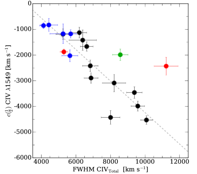
Fig. 3. Relation between the c(1/2) and the FWHM of the total CIV \lambda 1549 emission. Dashed gray line corresponds to the best fit using an orthogonal method. Black, blue, green and red filled circles correspond respectively to normal, BAL, mini-BAL and RL quasars for the GTC-xA sample.
