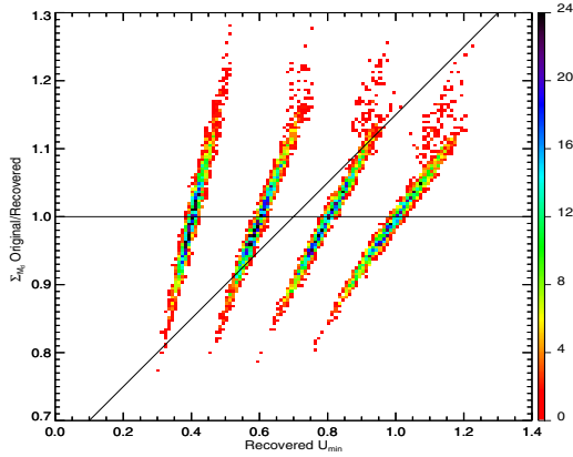
Fig. C.1. Comparison of the original and recovered dust mass under CIBA and instrumental noise simulation in the diffuse ISM for a 30' resolution. Colour corresponds to the density of points (see Fig. 5).
