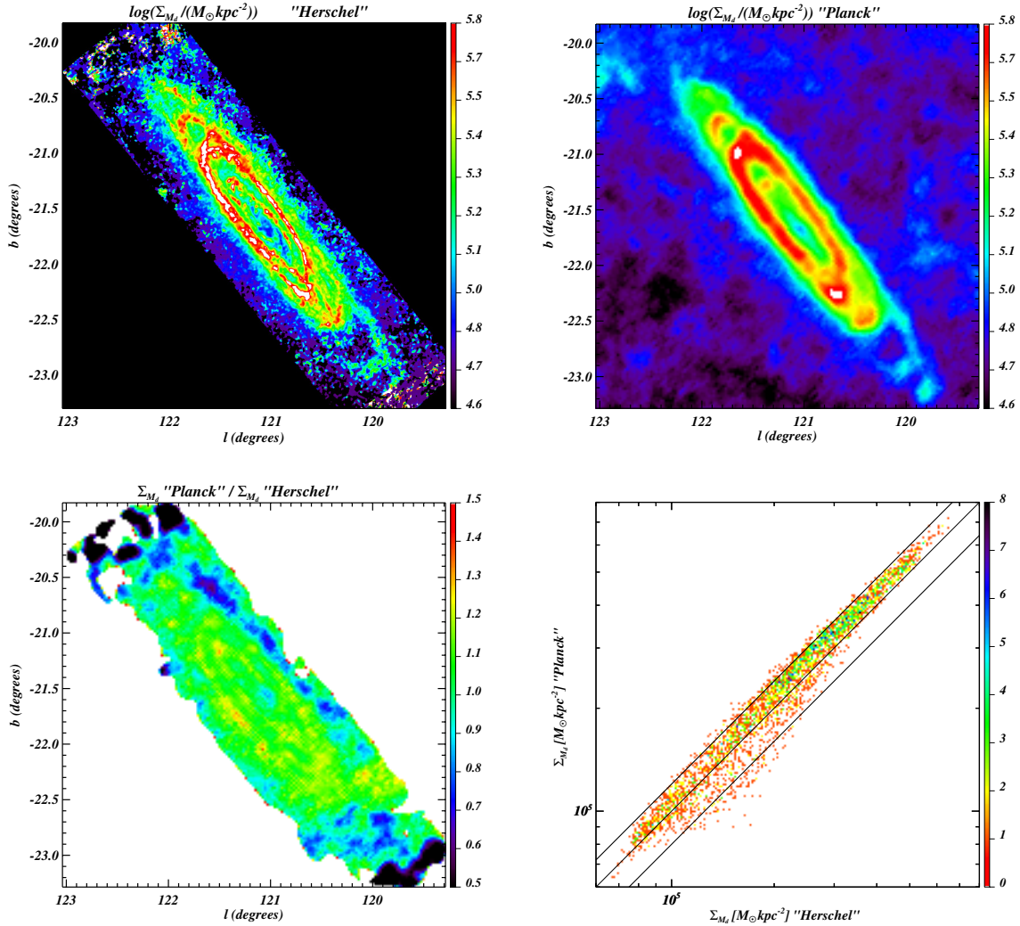
Fig. A.1. Comparison of M31 maps as seen by Herschel and Planck . The top row shows maps of the dust mass generated using Spitzer and Herschel data at high resolution ( left ) and the current estimates using IRAS and Planck data ( right ). The bottom row shows the ratio map of the two mass estimates (convolved to a common resolution and with the zero level matched) on the left, and their scatter on the right. The diagonal lines in the bottom right panel correspond to a one-to-one relationship and a \pm 20\% difference about that. The colour in the last panel corresponds to the density of points. Even though the two analyses are based on completely independent data, they agree remarkably well, differing by less than 10% across most of the galaxy.
