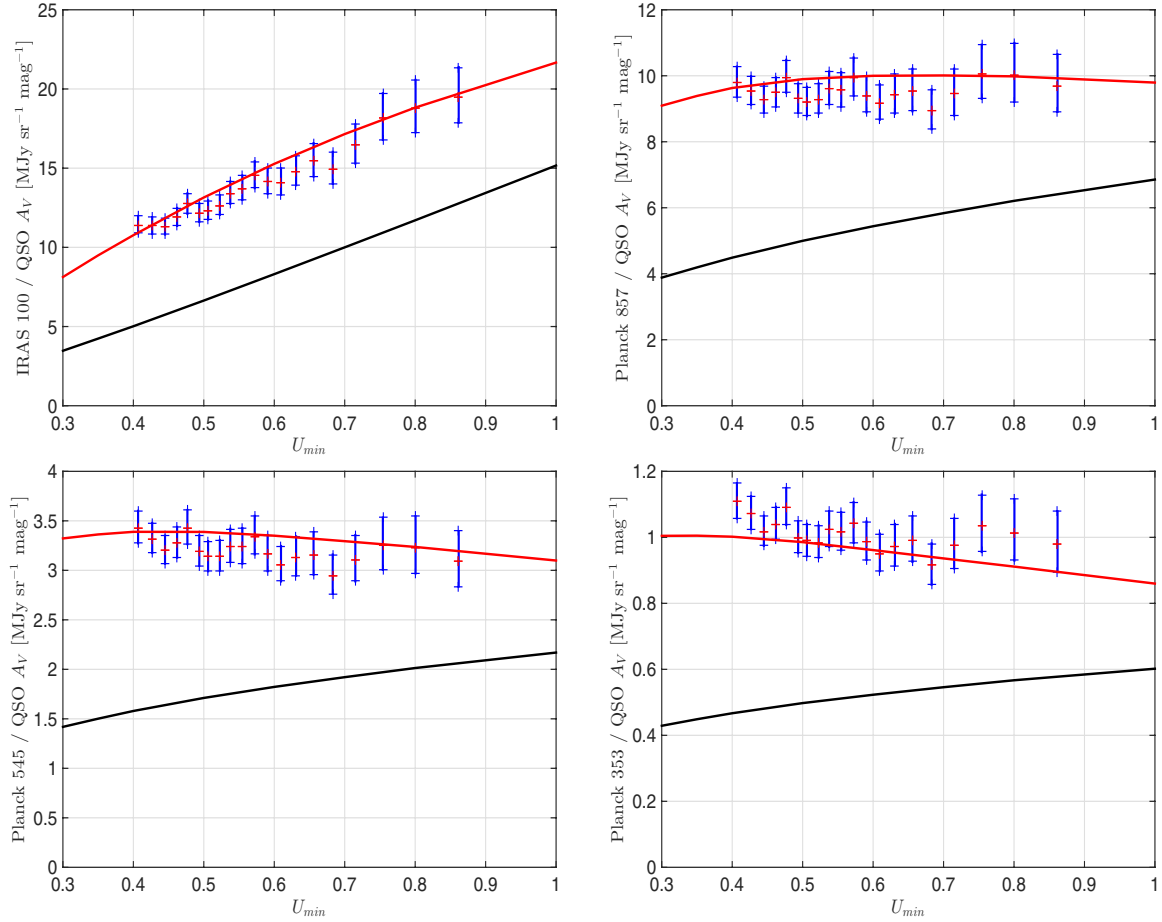
Fig. 12. Specific intensities per unit of optical extinction derived from a linear fit between the dust emission maps and A_{V,QSO} are plotted with red crosses and error bars in blue versus the fitted parameter U_{min} . The top row corresponds to IRAS 100 ( left ) and Planck 857 ( right ) and the bottom row to Planck 545 ( left ) and Planck 353 ( right ). The DL model values are plotted in black and the renormalized model in red. This plot shows that a U_{min} -dependent renormalization brings the DL model into agreement with the IRAS and Planck data.
