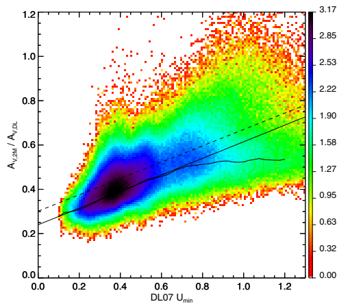
Fig. 16. Renormalization of the DL A_V values in molecular clouds. Pixels from the five molecular complexes with 1 < A_{V,2M} < 5 are included here. Colours encode the logarithm of the density of points (see Fig. 5). For each U_{\min} value, the solid curve corresponds to the best fit slope of the A_{V,DL} versus A_{V,2M} values. The straight solid line corresponds to a fit to the solid curve in the 0.2 < U_{\min} < 1.0 range, where each U_{\min} is given a weight proportional to the number of pixels that have this value in the clouds. The straight solid line provides the A_{V,RC} renormalization, and the dashed line that derived from the QSO analysis.
