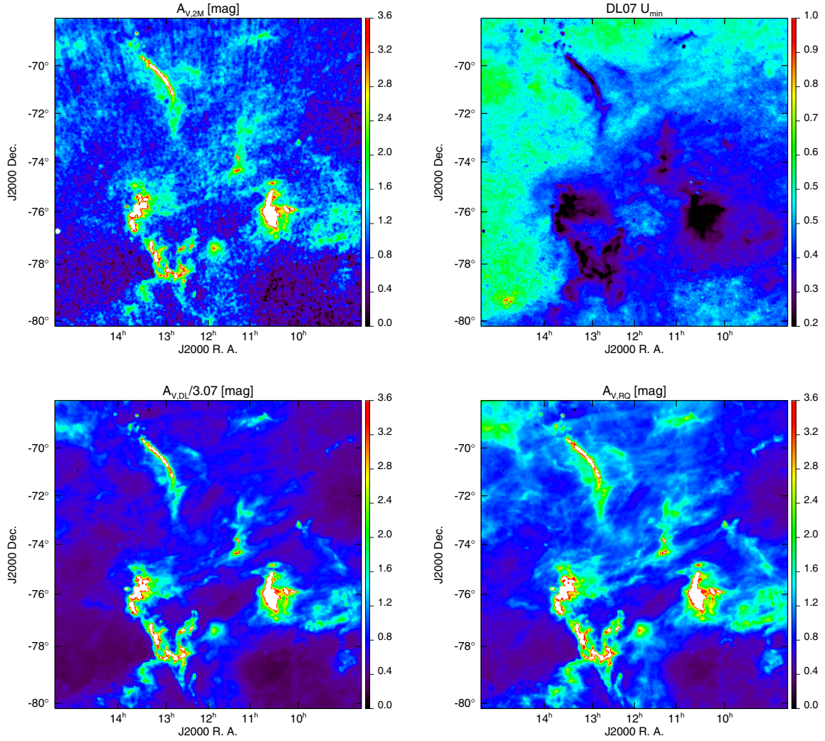
Fig. 13. 2MASS and DL estimates in the Chamaeleon cloud region. The top row shows the (background corrected) 2MASS A_{V,2M} map ( left ) and the DL U_{\min} map ( right ). The bottom row shows the DL A_{V,DL} estimate divided by 3.07 ( left ), and the renormalized model A_{V,RQ} estimates ( right ). (See Sect. 8.2 for a derivation of the 3.07 factor)
