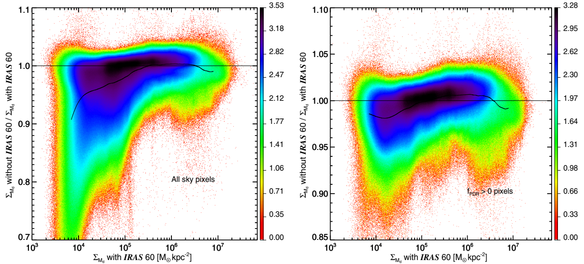
Fig. 6. Comparison between the dust mass estimates when the IRAS 60 constraint is excluded or included in the fit. The left panel shows all the sky pixels, and the right panel only the f_{\text{PDR}} > 0 pixels. The vertical axis corresponds to the ratio of the inferred mass density of a fit without using the IRAS 60 constraint to that obtained when this constraint is present (see text). Colour corresponds to the logarithm of the density of points (see Fig. 5). The curve corresponds to the mean value.
