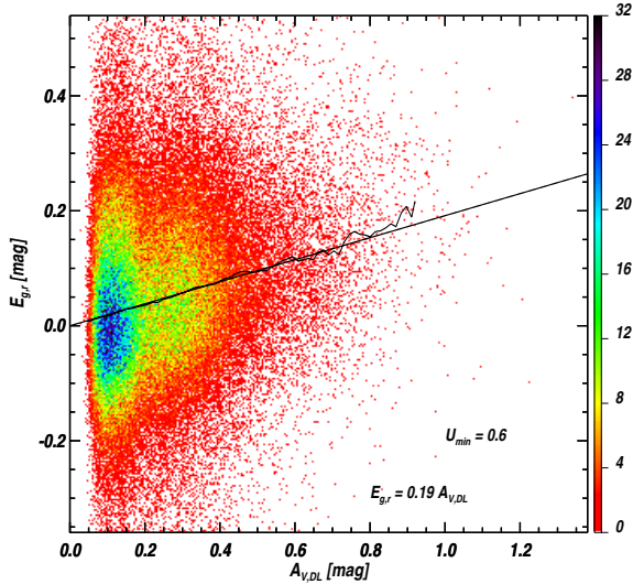
Fig. B.2. Colour excess E_{g,r} versus A_{V,DL} for the QSOs with U_{\min} = 0.6 . Colour corresponds to the density of points (see Fig. 5). The straight line corresponds to the best fit for all the QSOs. For each A_{V,DL} , the black curve corresponds to the mean E_{g,r} for the QSOs in an interval with a half-width \delta A_{V,DL} = 0.01 . Even though the QSOs show significant scatter, the E_{g,r} versus A_{V,DL} relationship is very linear; the mean E_{g,r} for each A_{V,DL} curve does not show significant departures from the straight line.
