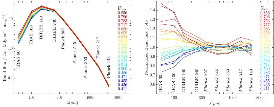
Fig. 11. FIR measured intensity per unit of optical extinction as a function of the fitted parameter U_{\min} . In the right panel , the SEDs are divided by the mean SED, i.e. normalized with the SED per unit of optical extinction obtained without binning on U_{\min} .
