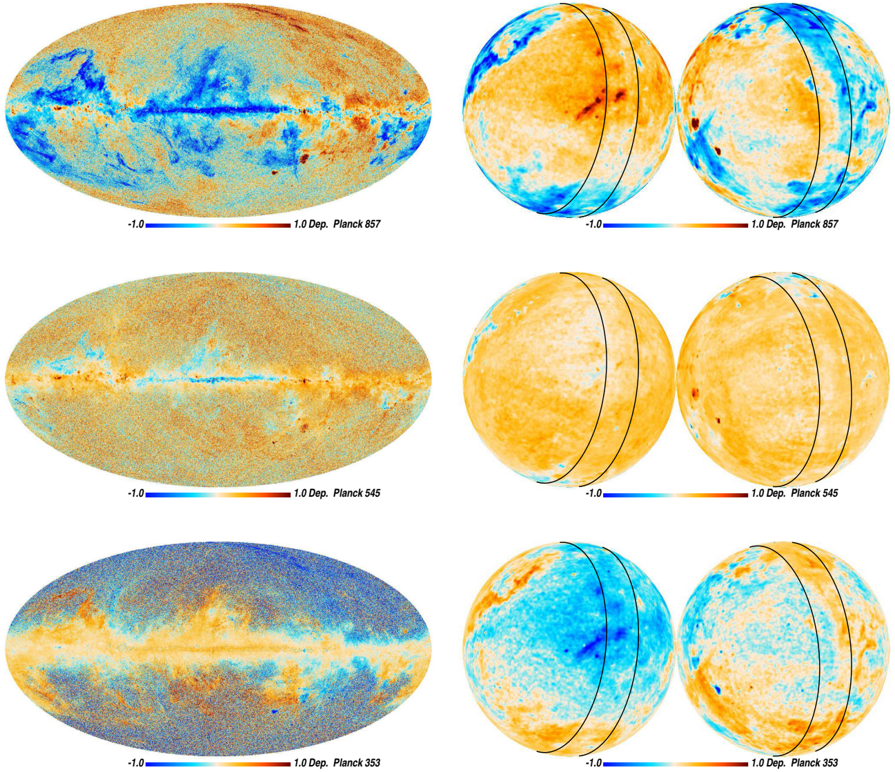
Fig. 4. Comparison between the model and the Planck data used to constrain the fit. Each panel shows the model departure from the data defined as \text{Dep.} = (\text{Model} - \text{Map}) / \text{Uncertainty} . The top row corresponds to Planck 857, the central row to Planck 545, and the bottom row to Planck 353. The polar projection maps are smoothed to 1^\circ resolution to highlight the systematic departures, and lines of Ecliptic latitude at \pm 10^\circ are added for reference.
