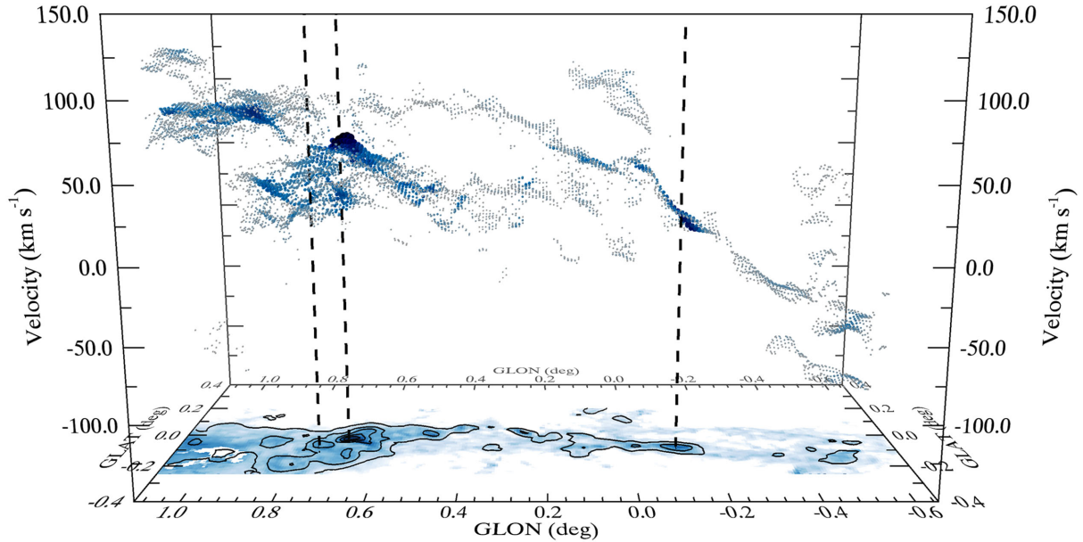
Figure 6. A PPV diagram highlighting the large-scale kinematic structure of the CMZ. Each pixel denotes the location and centroid velocity of a Gaussian component identified in HNC O emission and extracted using SCOUSE . The size (from small to large) and colour (from light to dark) of each data point is proportional to the peak intensity of the corresponding spectral component. At the base of the plot, in logarithmic colour-scale, is the Herschel -derived molecular hydrogen column density map (Battersby et al. in preparation). Column densities range from 10^{22} – 10^{24} \text{cm}^{-2} . Overlaid are contours highlighting the distribution of HNC O integrated emission. Contour levels are, 5, 25, 45, 65, and 85 percent of peak (integrated) emission (cf. Fig. 4). The three vertical dotted lines refer to the locations P1, P2, and P3, also highlighted in Fig. 4 (the corresponding spectra of which are shown in Fig. 3). A movie that shows this figure in 3D is available in the online supplementary material.
