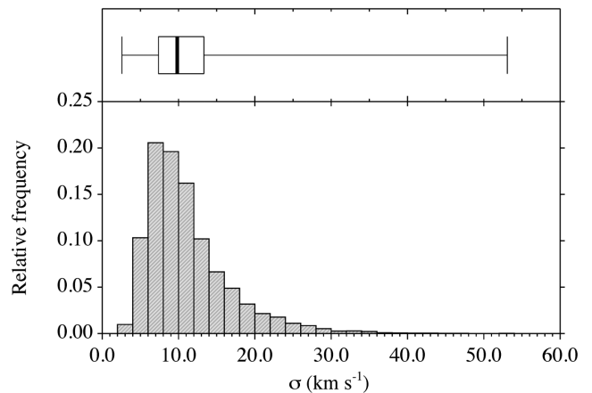
Figure 7. Top: a box plot of the velocity dispersion for all spectral components extracted from the HNC O spectral line data using SCOUSE . This highlights the range in velocity dispersion, the interquartile range (the box itself) and the median velocity dispersion ( \sim 9.8 \text{ km s}^{-1} , vertical thick black line). See Section 4.2.2 for more details. Bottom: a histogram of the velocity dispersion.
