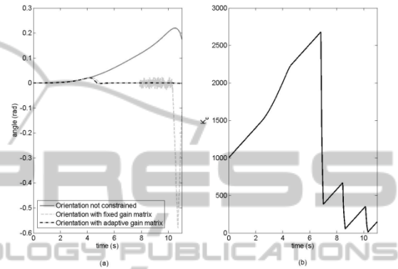
Figure 5: Trajectory example 3. Left: base yaw angle of not constrained, constrained (fixed K_c ) and fuzzy-adaptive trajectories. Right: calculated K_c adaptive value.
