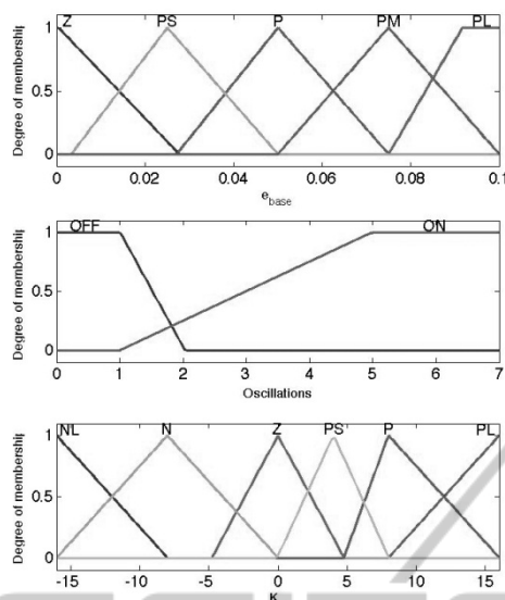
Figure 1: Fuzzy membership input and output functions. From left to right: (a) constraint error; (b) oscillation of joints; (c) output K_c .
