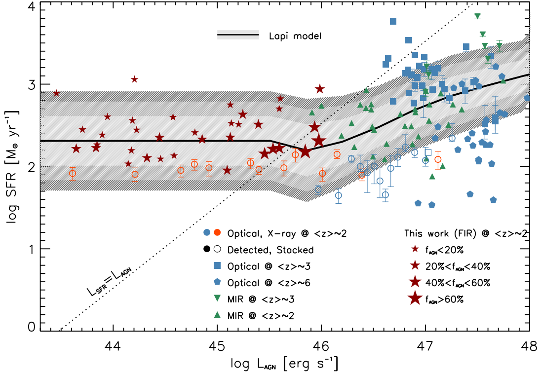
Figure 4. Co-evolution plane between bolometric AGN luminosity and SFR in the hosts z > 1.5 . The gray shaded areas show the average locus of the evolutionary tracks from the model of Lapi et al. (2018), adopting a SFR detection threshold around 10^2 M_\odot \text{ yr}^{-1} . Orange symbols refer to X-ray AGNs, green to mid-IR selected AGNs, blue to optically selected QSO. Complete references are reported in Bianchini et al. (2018). We include all SBs-AGN from our original sample (red filled stars): size of the symbol is proportional to the AGN luminosity contribution in the 5-40 \mu\text{m} range, derived from SED3FIT . SFR for the SBs in our sample is derived from L_{\text{IR}} in Table 1.
