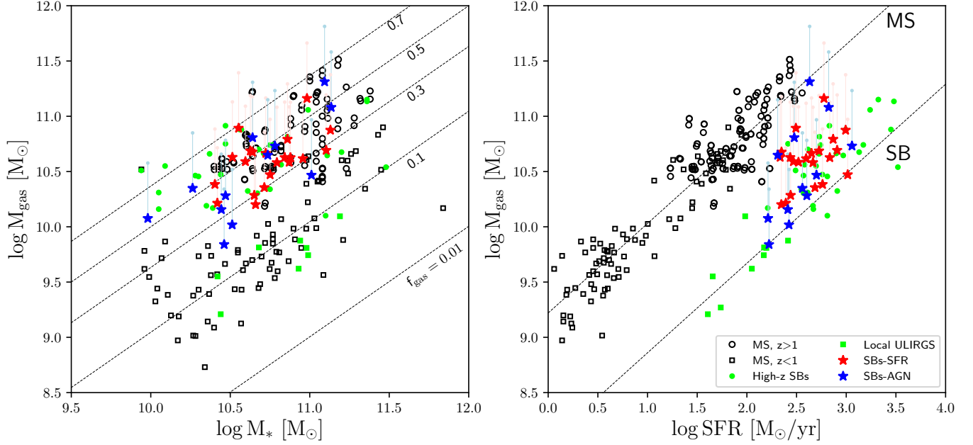
Figure 3. Left panel: M_{\text{gas}} versus M_{*} for the SBs with an ALMA detection (blue stars: SBs-AGN; red stars: SBs-SFR). M_{\text{gas}} are evaluated adopting a solar metallicity and an \alpha_{\text{CO}} of 0.8, corresponding to a DGR of 30, and represent our reference values; light points and relative connectors still refer to solar metallicity, but with \alpha_{\text{CO}} = 1.0 . Formal errors are smaller than the difference computed with the two methods. Loci of constant gas fraction (i.e. M_{\text{gas}}/(M_{\text{gas}} + M_{*}) ), are shown with dotted lines. Open black squares (circles) represent MS galaxies at z < 1 ( > 1 ) as compiled by Sargent et al. (2014) and Perna et al. (2018). Green symbols show local ULIRGs (filled squares) and high- z starbursts (filled circles). Right panel: M_{\text{gas}} versus \text{SFR} . Empirical model curves (dashed lines) for MS and ULIRGs/SB are described in Sargent et al. (2014).
