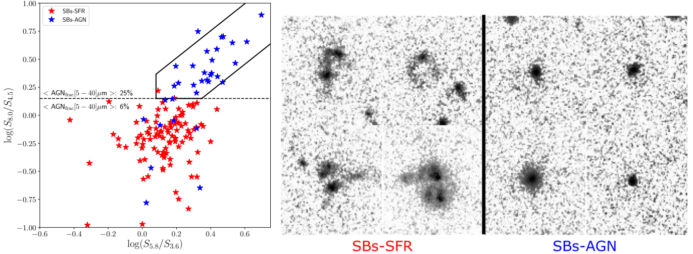
Figure 2. Left panel: Colour-colour IRAC plot of the 152 SBs selected in COSMOS. Blue stars are classified as SBs-AGN (35 in total), red stars as SBs-SFR (117). Black lines mark the position of the AGN selection criteria from Donley et al. (2012). The mean value of the sample AGN contribution (in percentage units) between [5-40]\mu\text{m} over and below this value is reported. Right panel: Morphological examples of SFR dominated starbursts (left) and AGN dominated starbursts (right). HST-ACS cutouts have a size of 5'' \times 5'' .
