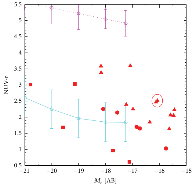
FIGURE 3: The CMD (NUV- r ) versus M_r of the CVnI Cloud members. The Wyder et al. [25] fits of the blue and red sequences (cyan/magenta lines) are plotted, including their error bars. The oval indicating the position of UGC 7639 also includes UGC 7408, a galaxy slightly bluer and brighter than our dwarf. Different symbols correspond to different SFRs: squares are for \text{SFR} \geq 0.1 M_\odot/\text{yr} , triangles for \text{SFR} \leq 0.05 M_\odot/\text{yr} , and circles for SFRs in between.
