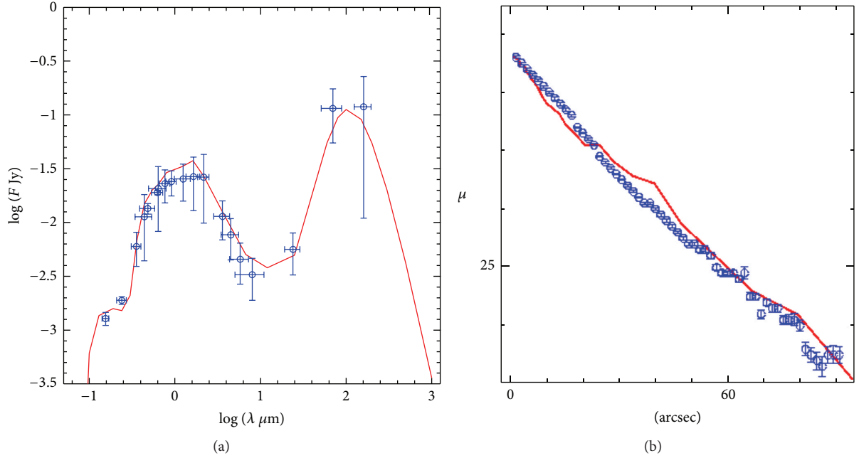
FIGURE 5: (a) the SED of UGC 7639. Blue filled circles correspond to UV/Optical/IR/FIR data, in particular FUV and NUV total fluxes from Table 1, u, g, r, i, and z, fluxes from NASA-Sloan Atlas [29], B and R from Bremnes et al. [20], and IR and FIR from Dale et al. [53]. Error bars account for bandwidth and 3\sigma flux uncertainties. The solid (red) line shows the prediction of our model (see text). (b) the r-band luminosity profile of our simulated image in Figure 4 is compared with that measured in the same band and shown in Figure 2. Error bars <1\% do not appear in the figure.
