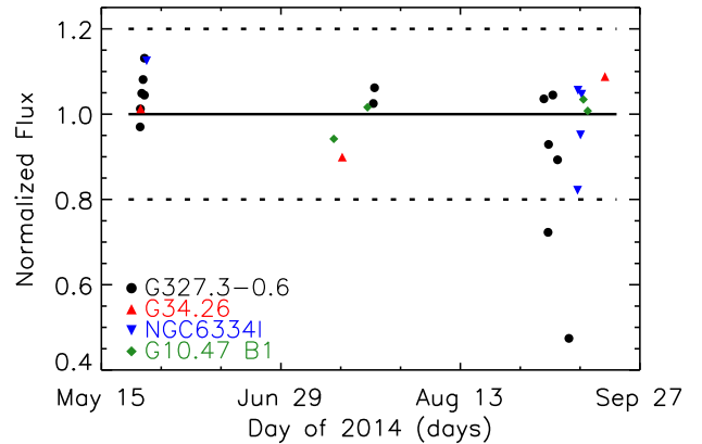
Fig. 1: Ratio of the daily integrated flux to the average flux of the CO (6–5) transition for the calibration sources observed during the campaign. A solid horizontal line is placed at 1.0 and the dashed lines indicate a deviation of 20% from unity.
