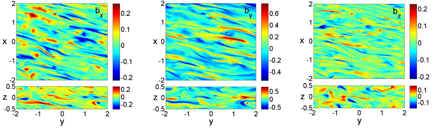
Figure 4. Typical structure of the magnetic field in the fully developed quasi-steady turbulent state at t = 550 for the box (4, 4, 1) . Shown are the sections in the (y, x) and (y, z) planes.
