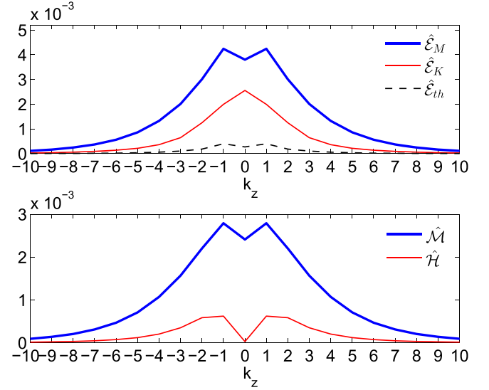
Figure 5. Integrated in the (k_x, k_y) plane are the time-averaged kinetic, \hat{\mathcal{E}}_K , magnetic, \hat{\mathcal{E}}_M , and thermal, \hat{\mathcal{E}}_{th} , energy spectra (upper panel) as well as Reynolds, \hat{\mathcal{H}} , and Maxwell, \hat{\mathcal{M}} , stresses (lower panel) as a function of k_z for the box (4, 4, 1) .
