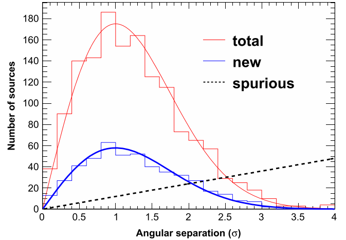
Figure 4. Distributions of normalized angular separation between 3LAC sources and their assigned counterparts. The normalization factor \sigma is defined in the text. Red: total. Blue: new sources. The curves correspond to the expected distribution for real associations and the dashed line illustrates that expected for spurious associations.
