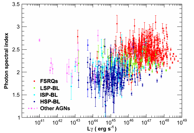
Figure 14. Photon index vs. gamma-ray luminosity. Red: FSRQs; green: LSP-BL Lacs; light blue: ISP-BL Lacs; dark blue: HSP-BL Lacs; magenta: other AGNs (circles: NLSy1s; squares: radio galaxies; up triangles: SSRQs; down triangles: AGNs of other types).
