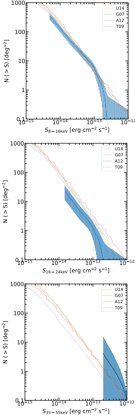
Figure 3. From top to bottom: \log N - \log S for the H1, H2 and upper limits for the VH band, compared with some population synthesis models (in dotted lines: orange, Ueda et al. 2014; green, Gilli et al. 2007; red, Akyas et al. 2012; violet, Treister et al. 2009). The uncertainties are Poissonian, and take into account a rough constant 13% of cosmic variance in the H1 band. In the bottom panel, the dashed black line denotes where the upper limit would lie adopting lower reliability thresholds, appropriate for the two tentative detections.
