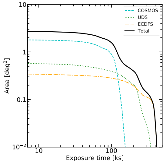
Figure 1. Area as a function of FPMA+FPMB exposure for the three field considered in this work (COSMOS, dashed cyan; UDS, dotted green; ECDFS, dot-dashed orange). The summed area curve is shown as the thick black line, for a total area of 2.74 \text{ deg}^2 .
