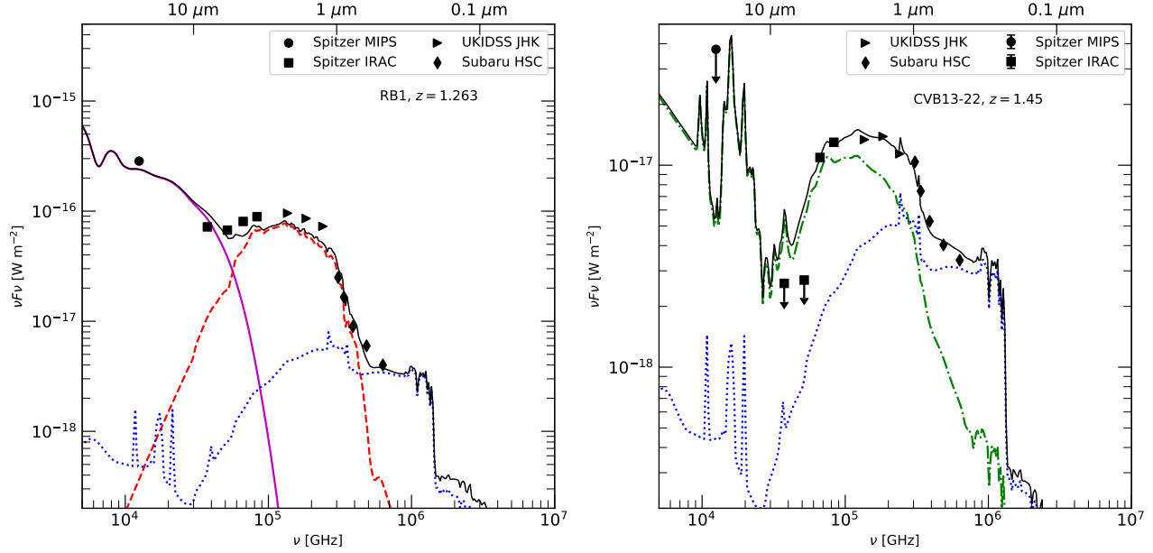
Figure 5. Optical/IR SEDs of RB1 (left) and CVB13-22 (right), the two possible counterparts to the NuSTAR detection in the UDS field. The circle datapoint is Spitzer MIPS, the squares refer to Spitzer IRAC, the rightward triangles to UKIDSS in the JHK bands, and the diamonds to Subaru HSC in the g, r, i, z, Y bands. The optical-IR part of the SED is fitted with an AGN (solid violet), passive (dashed red), late-type (dot-dashed green) and star-forming (dotted blue) templates. Upper limits are labeled as downward arrows, and have been estimated considering the minimum flux of the sources detected by one instrument in the surroundings of the target. While the AGN component in the SED in RB1 is heavily reddened ( E(B - V) \sim 6.2 ), giving support to the classification of obscured (possibly CT) AGN, the same component in CVB13-22 is not required by the fit.
