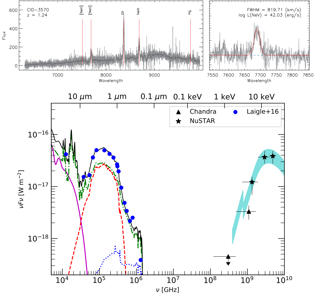
Figure 4. Top. DEIMOS spectrum of cid_3570 (Hasinger et al. 2018), with the right panel zooming on the NeV emission line. Bottom. Broadband SED for cid_3570, the interesting source at z = 1.244 in the COSMOS field significantly detected in the H1 band by NuSTAR . The optical-IR part of the SED is fitted with an AGN (solid violet, Assef et al. 2010), passive (dashed red, Assef et al. 2010), late type (dot-dashed green, Kirkpatrick et al. 2015), and star-forming (dotted blue, Assef et al. 2010) templates. Data points (blue circles) are from the catalog of Laigle et al. (2016), and references therein. In the X-ray part of the SED, the Chandra (triangles) soft (0.5 – 2 keV) band flux is an upper limit. The NuSTAR fluxes derived from the spectral analysis are labeled with stars. Uncertainties on \nu F_\nu are at 1\sigma confidence level, and the cyan region is the pexrav (Magdziarz & Zdziarski 1995) model ( \pm 1\sigma ) adopted to derive the NuSTAR fluxes.
