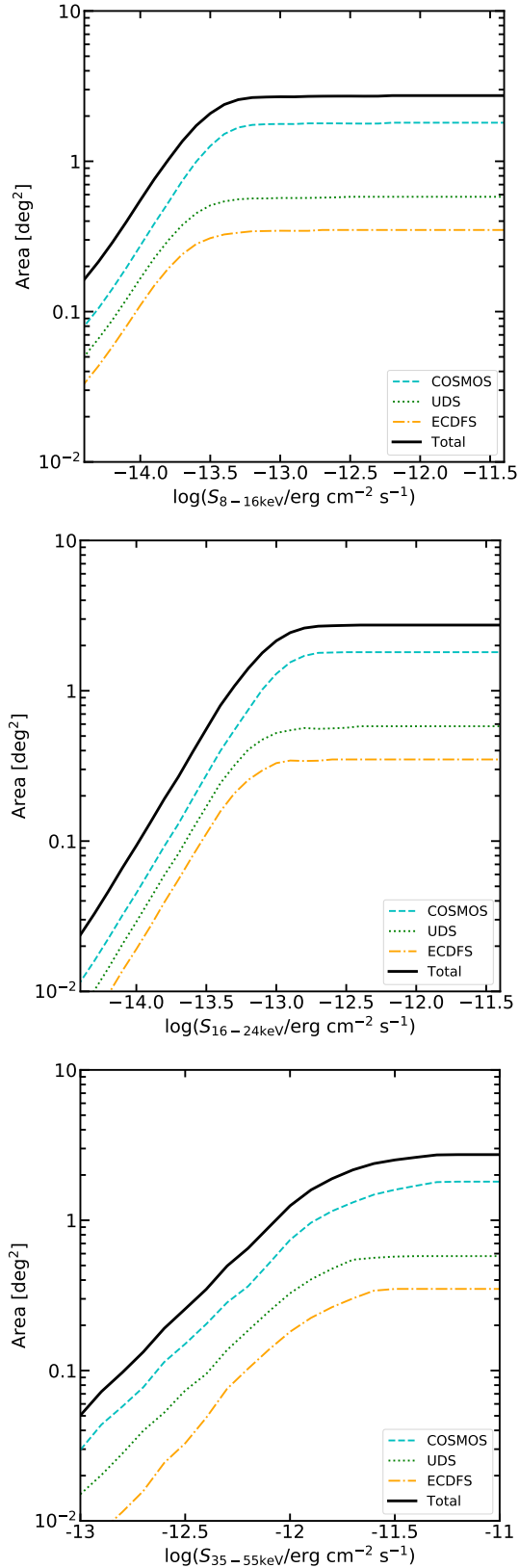
Figure 2. From top to bottom: sensitivity for the H1, H2, and H3 band, respectively. In each panel, the COSMOS curve is shown by the cyan dashed line, the UDS one in dotted green, and the ECDFS one in dot-dashed orange. The total curve is the black thick line.
