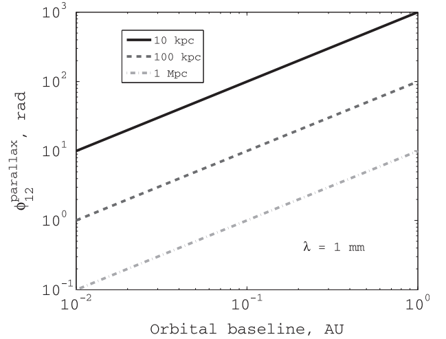
Fig. 4. Interferometric parallax phase \phi_{12}^{parallax} estimation for different target object distances for a wavelength \lambda = 1 \text{ mm} . The parameter space below the 10 kpc line has never been probed through direct distance estimation methods. (Logarithmic scale.)
