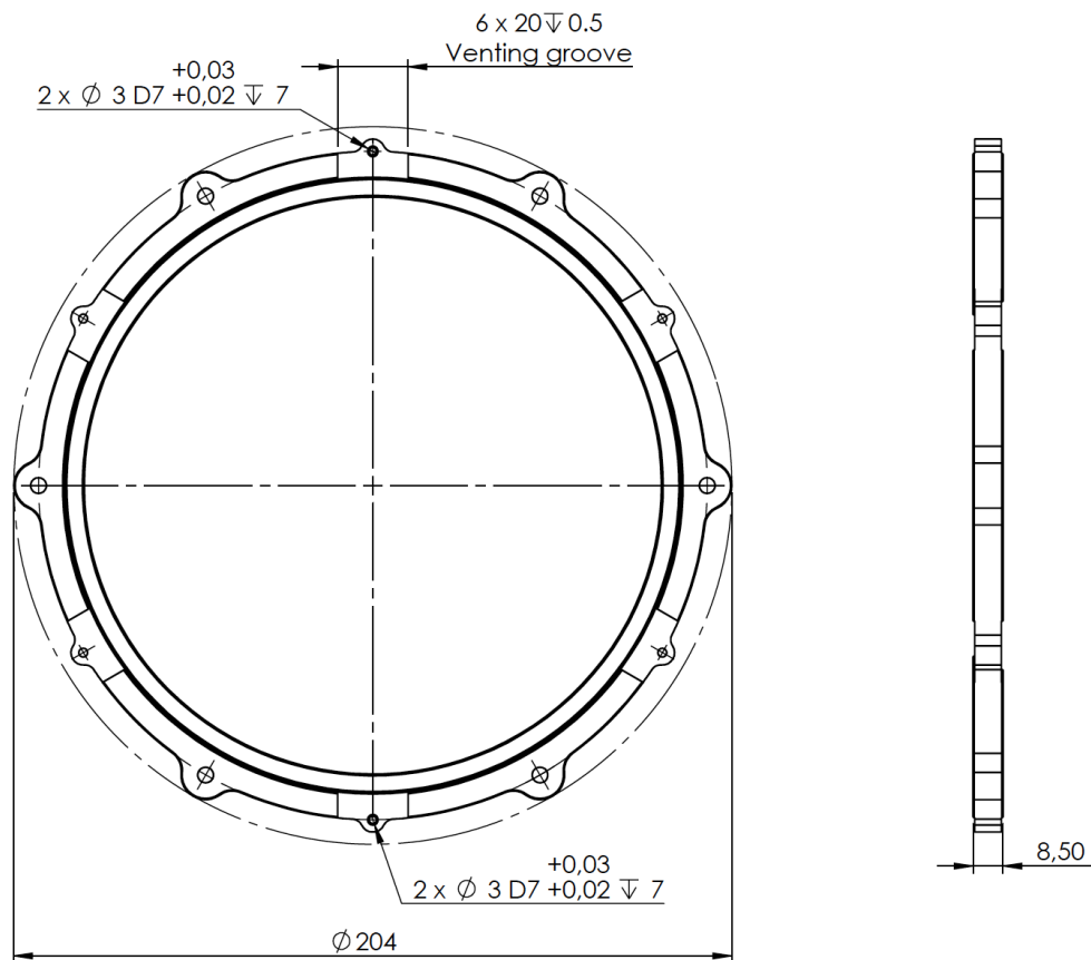
Fig. 3 – Custom frame of a X-IFU filter wheel optical blocking filter.
