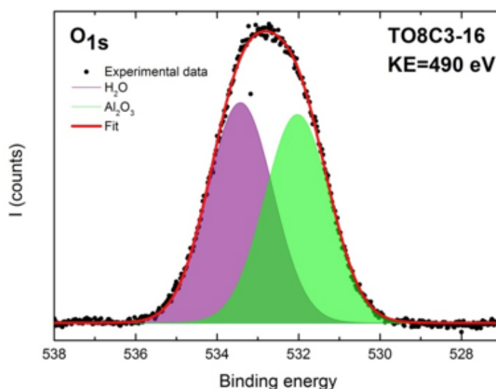
Fig. 10 – Fit for the O 1s peak with KE of 490 eV of the sample TO8-C3-16. Data reported are experimental (black full circle), best fit (red line), O of \text{H}_2\text{O} component (purple filled curve, and O of \text{Al}_2\text{O}_3 (green filled curve).
