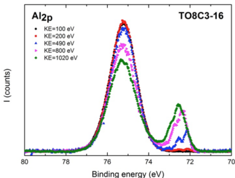
Fig. 7 – Normalized XPS measurements of the irradiated sample, the TO8C3-16 filter. The Al 2p peak acquired at different KE of the outgoing electron 100 eV (black), 200 eV (red), 490 eV (blue), 800 eV (magenta) and 1020 eV
