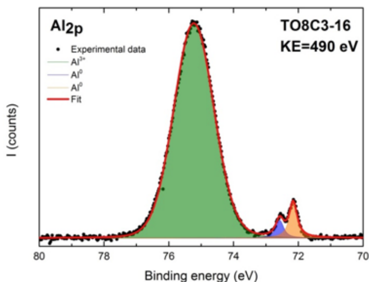
Fig. 9 – Fit for the Al 2p peak with KE of 490 eV of the irradiated sample TO8C3-16. Data reported are experimental (black full circle), best fit (red line), \text{Al}^{3+} 2p component (dark green filled curve), \text{Al}^0 2p 1/2 (blue filled curve), and \text{Al}^0 2p 3/2 (orange filled curve).
