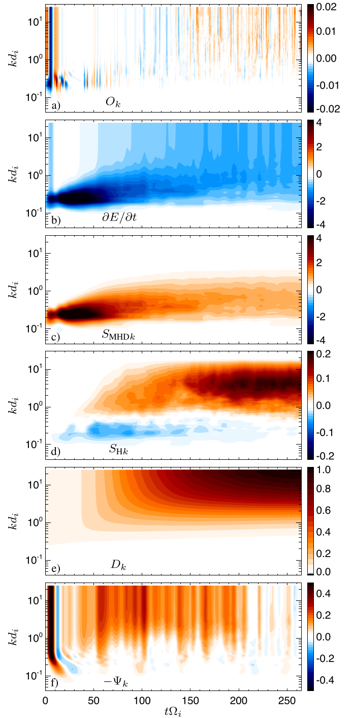
Figure 5. Evolution of the compressible ST law: color scale plots of (a) O_k , (b) \partial E_k / \partial t / 4 , (c) S_{\text{MHD}k} , (d) S_{\text{H}k} , (e) D_k , and (f) -\Psi_k as functions of time and k . All the terms are given in units of the total heating rate Q .
