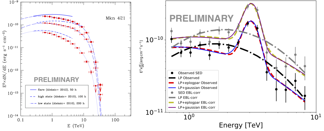
Figure 2: Left panel: simulations of different source states of Mkn 421. Depending on the source state, 50 h (red dots), 100 h (red triangles) and 200 h observations (red squares) were simulated respectively, considering the intrinsic source spectra (see legend) convolved with the EBL absorption [19] (blue dot-long-dashed, long-dashed and dotted lines). Right panel: short-duration (1 h exposure) simulation of the Mkn 501 \gamma -ray narrow spectral feature in the high state. Both observed and EBL-corrected spectra are shown.
