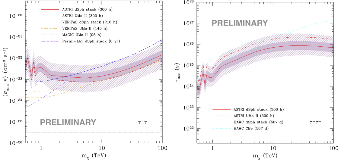
Figure 4: Comparison between 300 h ASTRI MA sensitivity limits to DM particle cross section ( left panel ) and lifetime ( right panel ) for the \tau^+\tau^- channel ( red solid and dashed lines ), and the corresponding limits obtained by existing space- and ground-based facilities for \gamma -ray observations (see legends for color and line-style codes). Error bands at 68% probability on the parameters due to photon statistics ( pink shaded areas ) and to uncertainties on the DM amount in the dSph halos ( pink hatched areas ) are indicated. The velocity-averaged thermal relic cross section \langle\sigma v\rangle \sim 3 \times 10^{-26} \text{ cm}^3 \text{ s}^{-1} for DM annihilation [27] ( black dot-dashed line ) is indicated.
