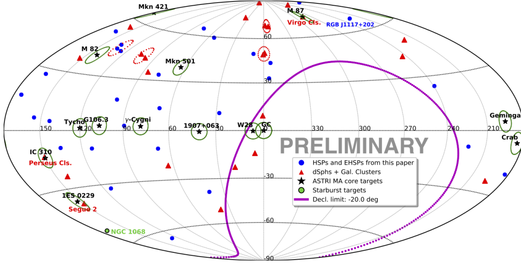
Figure 1: Sky distribution, in Galactic coordinates and Hammer-Aitoff projection, of the ASTRI MA extragalactic targets (see legend). The position in Galactic coordinates of the ASTRI core-science targets (black stars) is also shown. A 5^\circ radius circle is drawn around clustered extragalactic targets to be potentially observed in a single joint observation (red dotted circles; see text). Core-science targets are also highlighted (green solid circles). The assumed limit on source declination for targets visible from the Observatorio del Teide (purple line) is indicated.
