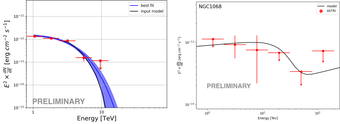
Figure 3: Left panel: spectrum of RGB J1117+202 for 200 h observations. The adopted source spectral model (black line) is shown superimposed to the corresponding uncertainty of the reconstructed emission profile (blue line and shaded area) and the observed spectrum (red dots). Right panel: simulated \gamma -ray spectrum of NGC 1068. The observed signal after 200 h of observation (red dots) is shown superimposed to the spectrum predicted by the AGN wind model (black line) [16, 17].
