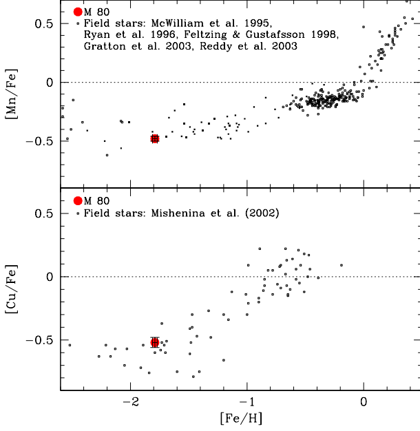
Fig. 17. [Mn/Fe] (upper panel) and [Cu/Fe] (lower panel) average ratios of M 80 from stars with UVES spectra compared with various samples of field stars as a function of metallicity. The rms scatter for Mn, Cu, and Fe are plotted for M 80 (they are inside the large symbol).
