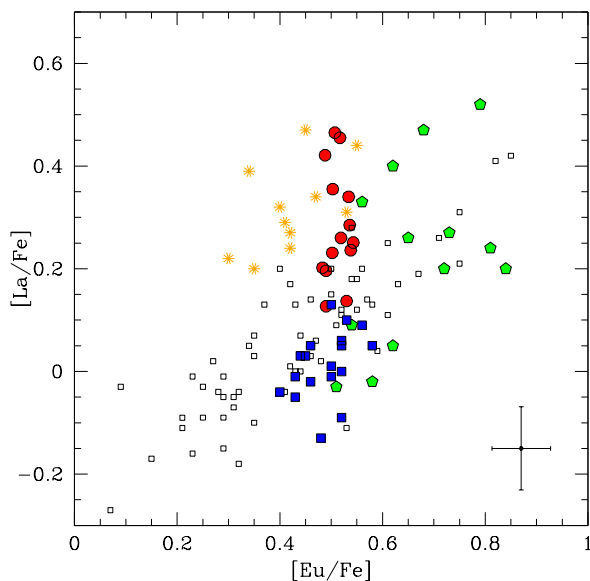
Fig. 21. [La/Fe] ratios as a function of [Eu/Fe] ratios for individual stars in M 80 (large filled circles) compared to r -only field stars from Roederer et al. (2010; small empty squares) and to GCs with a dispersion in s -process elements. Blue-filled squares indicate the r -only component in M 22 from Marino et al. (2011), orange asterisks are used for the r+s component in M 22 (see Roederer et al. 2011, Marino et al. 2011), and green-filled pentagons are giants in NGC 1851 from Carretta et al. (2011b). The internal error bars refer to our present analysis of M 80.
