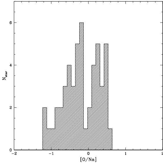
Fig. 8. The distribution of the [\text{O}/\text{Na}] ratios in M 80.
