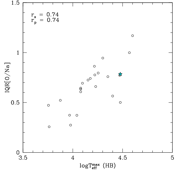
Fig. 16. Extension of the Na-O anti-correlation (measured using IQR[O/Na] ) as a function of the maximum temperature along the HB, taken from Recio-Blanco et al. (2006). M 80 is represented by a filled star symbol. The Spearman rank and the Pearson linear correlation coefficients are listed.
