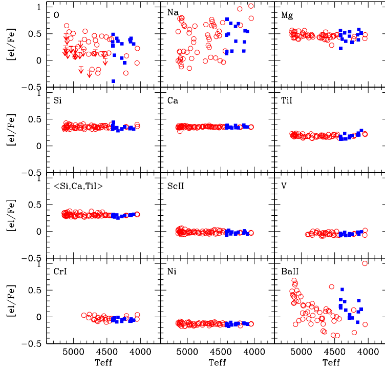
Fig. 6. Abundance ratios [\text{el}/\text{Fe}] as a function of T_{\text{eff}} for all stars in our sample. Filled squares and open circles indicate stars with UVES and GIRAFFE spectra, respectively. Internal error bars are listed in Tab. A.1 and Tab. A.2 in the Appendix.
