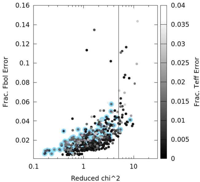
Figure 3. Fractional uncertainty on F_{\text{bol}} from the SED fitting procedure as a function of \chi^2_\nu and of T_{\text{eff}} uncertainty. The vertical line represents the cutoff of \chi^2_\nu \leq 5 for which the uncertainty on F_{\text{bol}} is at most 6% for most stars, thus permitting a determination of R_* to \approx 3\% . Points with blue haloes represent stars with transiting planets. Reproduced from Stassun et al. (2017a).
