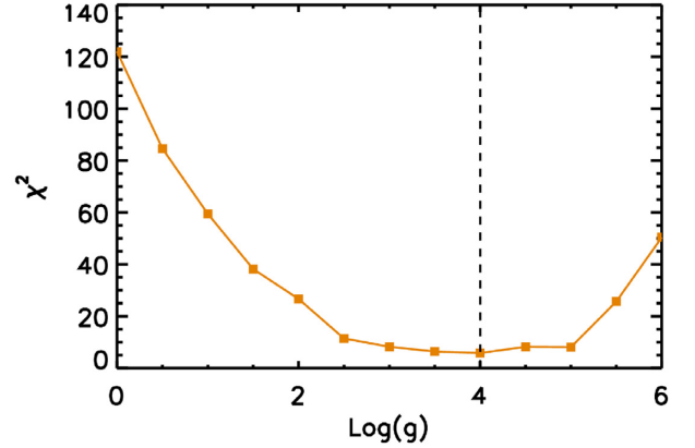
Figure 5. Values of the \chi^2 obtained from the fit versus the values of \log g for a fixed T_{\text{eff}} of 2800 K. The vertical dashed line highlights the position of the minimum of the curve.
