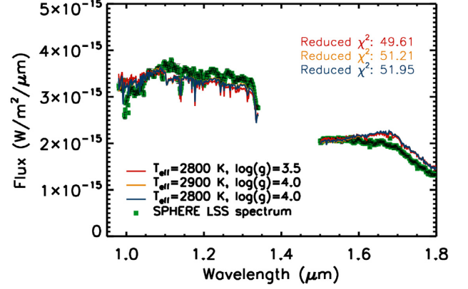
Figure 4. Comparison of the extracted spectrum for HD 1160 B (green squares) with the three best-fitting theoretical BT-Settl spectra (orange, red, and blue solid lines).
